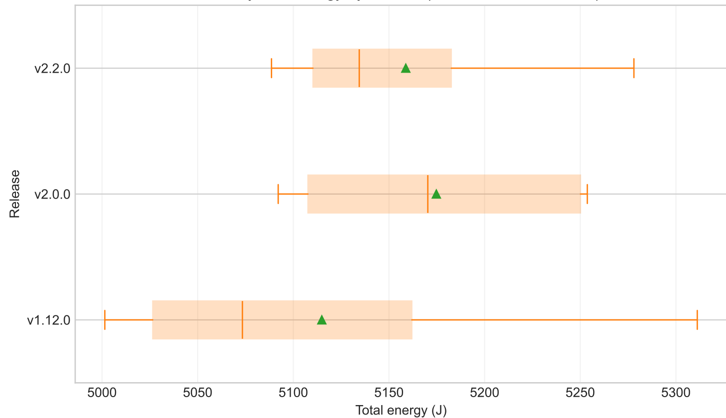
Total system energy by release (ec2, workload=medium)
