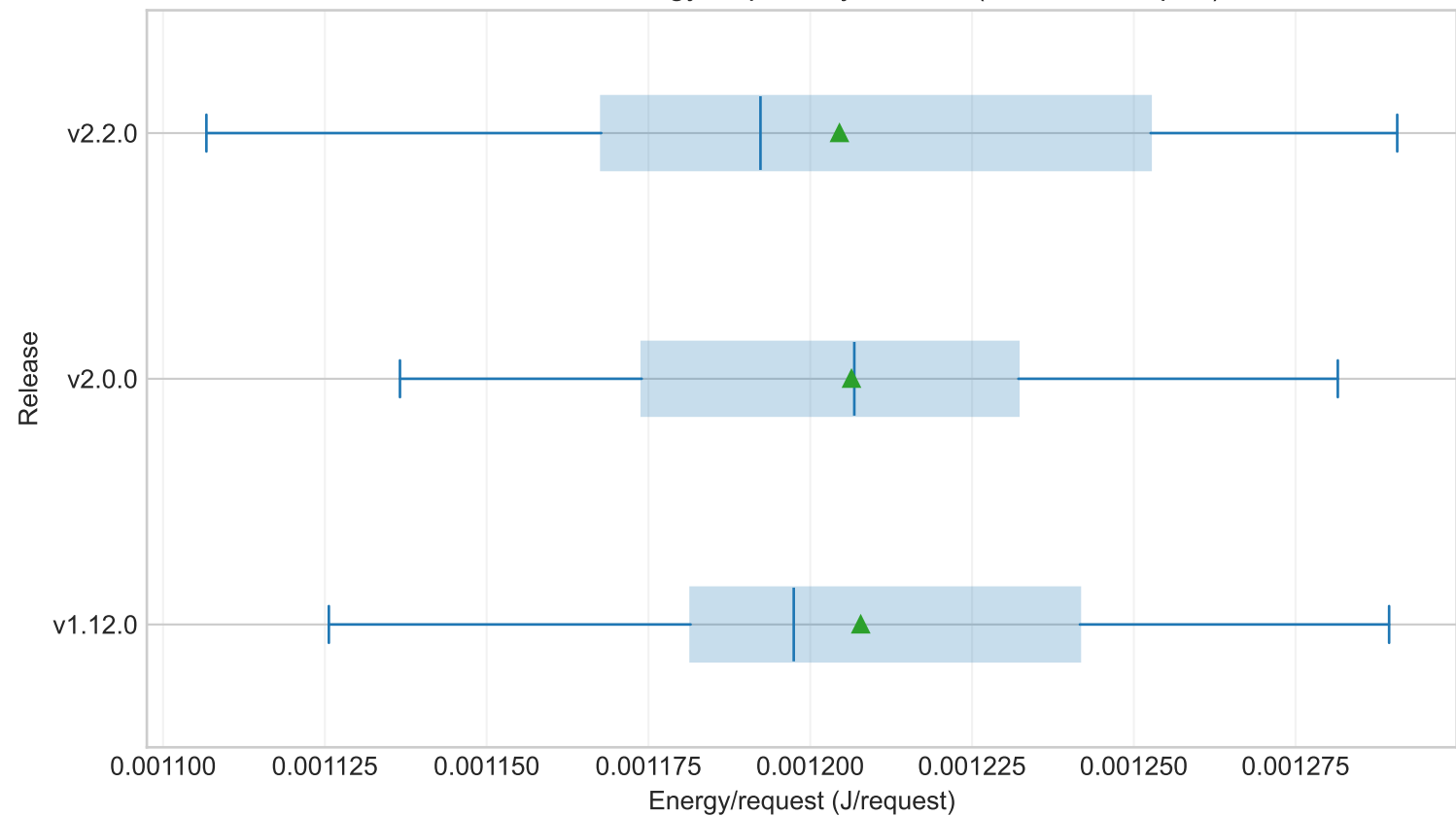
Fixed-utilisation energy/request by release (workstation, p80)
