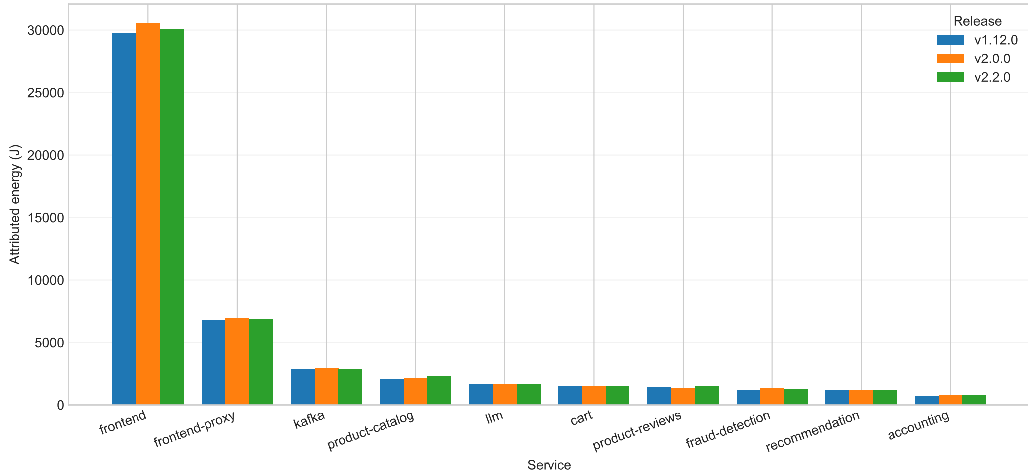
Service-level attributed energy by release (ec2, workload=medium, model=M1)
