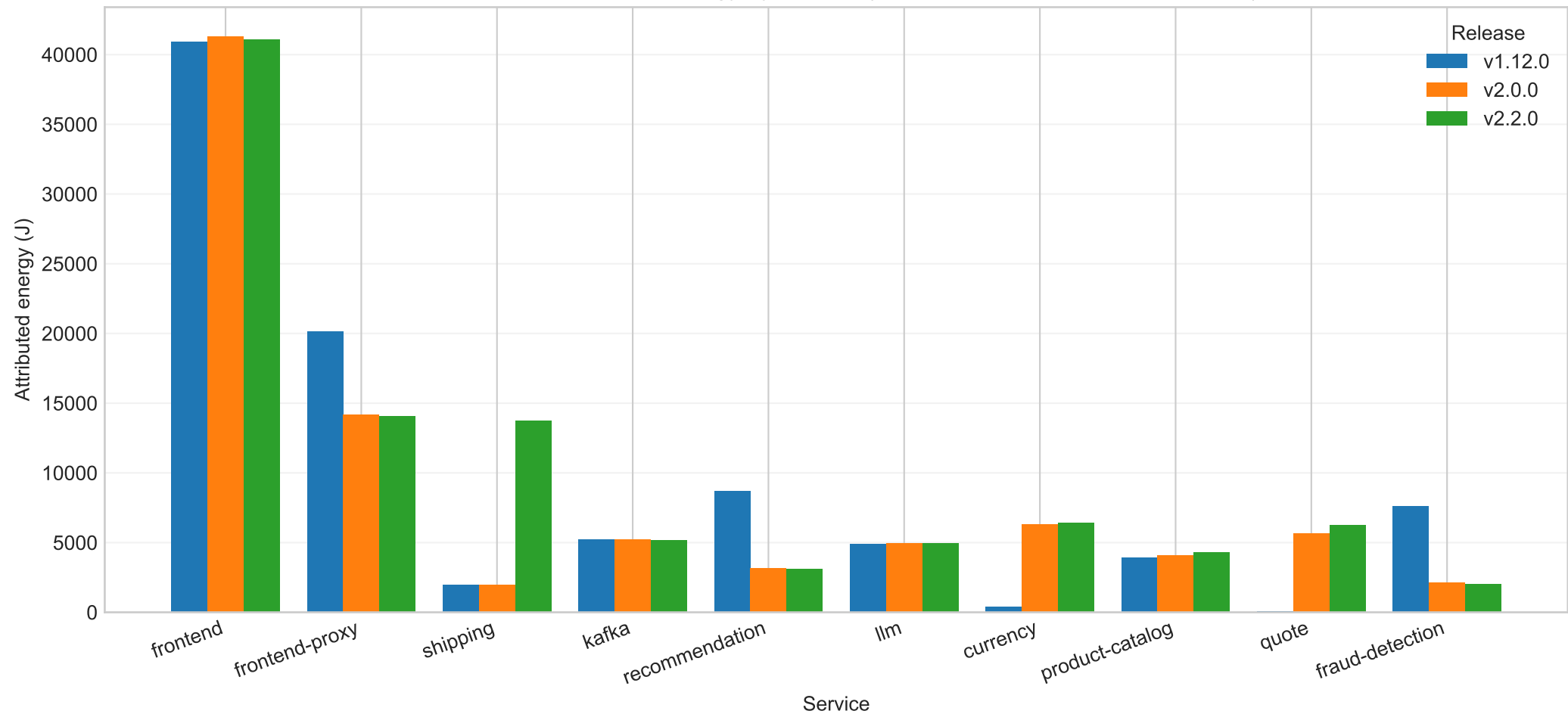
Service-level attributed energy by release (ec2, workload=medium, model=M2)
