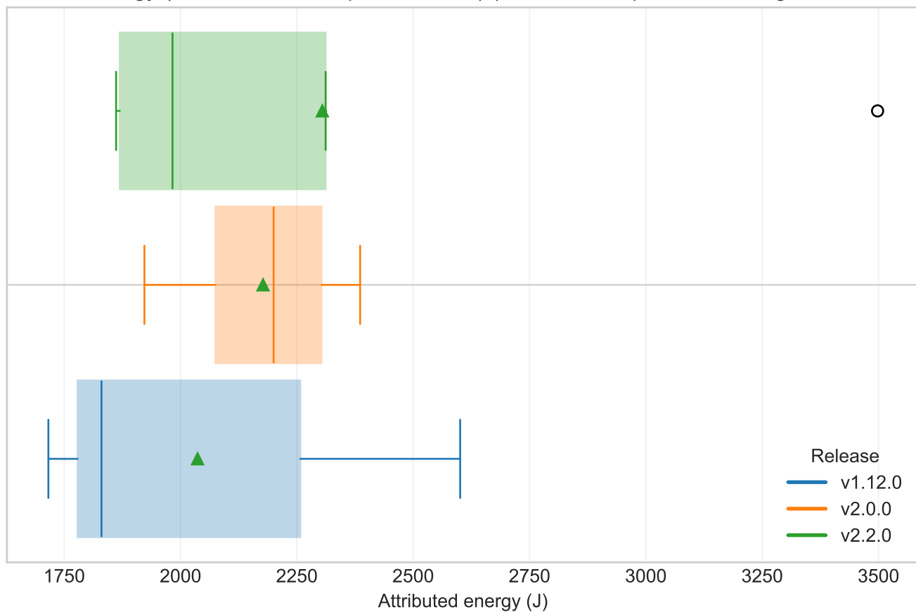
Selected service attributed energy (iteration-level boxplots, rotated) (ec2, service=product-catalog, workload=medium, model=M1)
