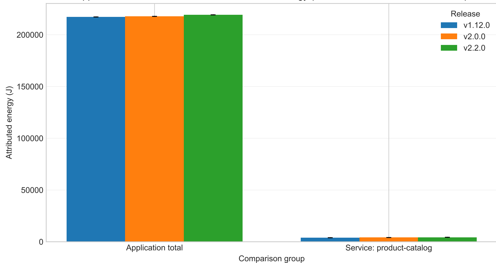
Application total vs selected services attributed energy (ec2, workload=medium, model=M2)
