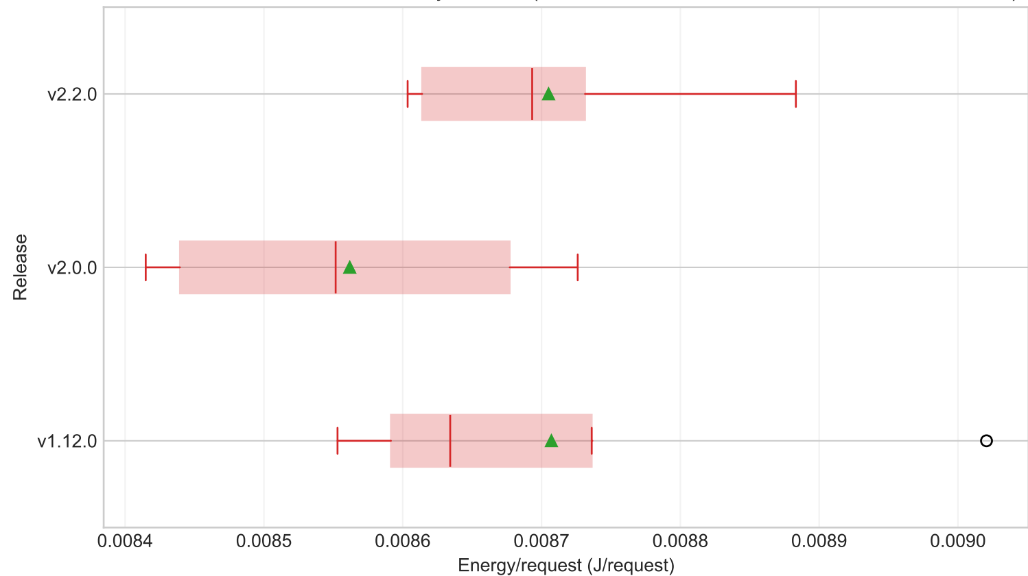
Fixed-util selected service EPR by release (ec2, service=cart, workload=medium, model=M1)
