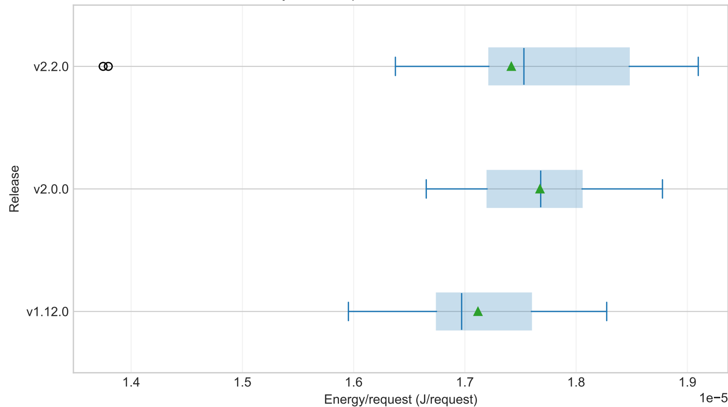
Fixed-util selected service EPR by release (workstation, service=cart, workload=medium, model=M1)
