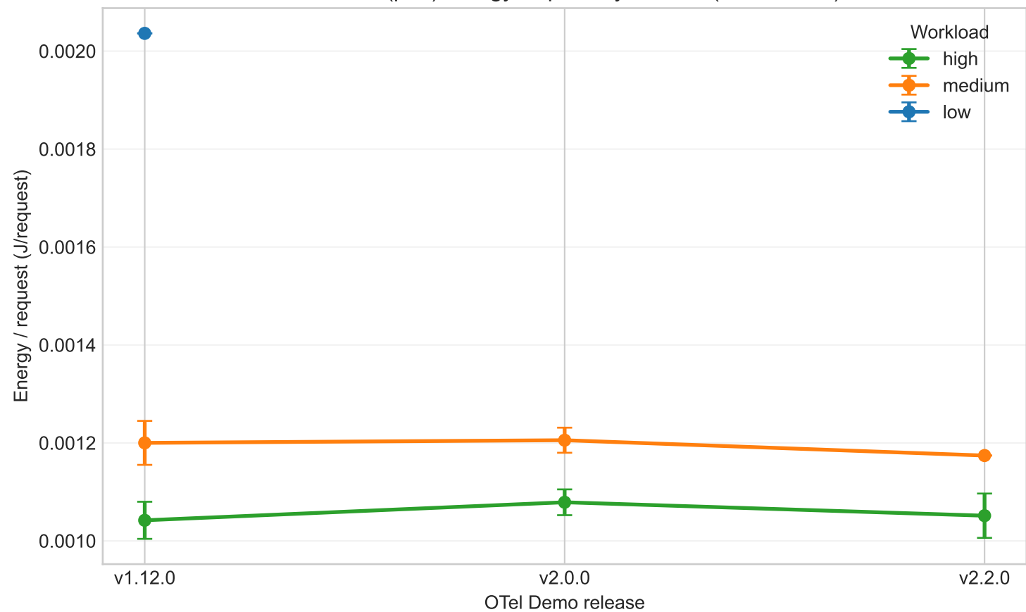
Fixed-util (p50) energy/request by release (workstation)
