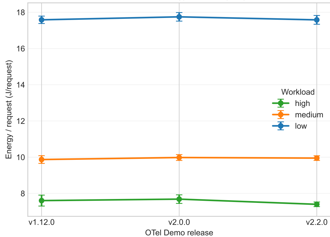
Calibrated energy/request (ec2)
