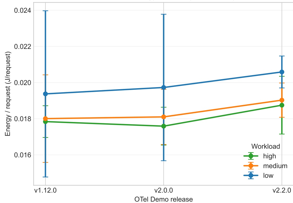
Calibrated energy/request (workstation)
