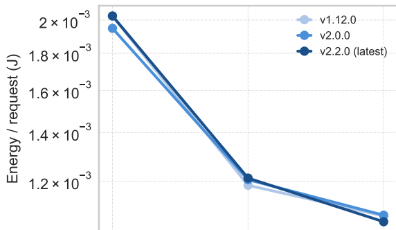
Social Network
