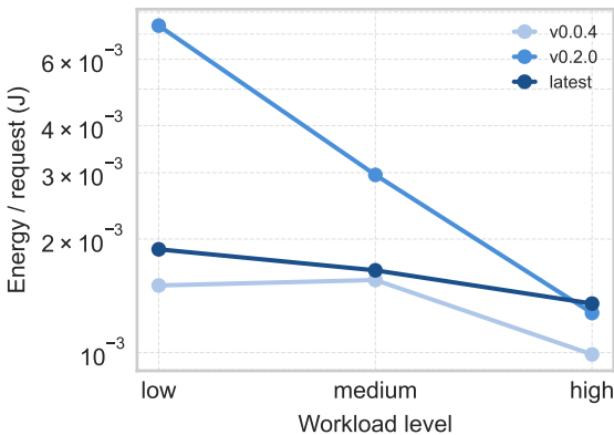
Train Ticket
