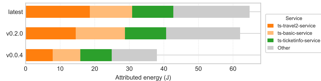
Train Ticket
