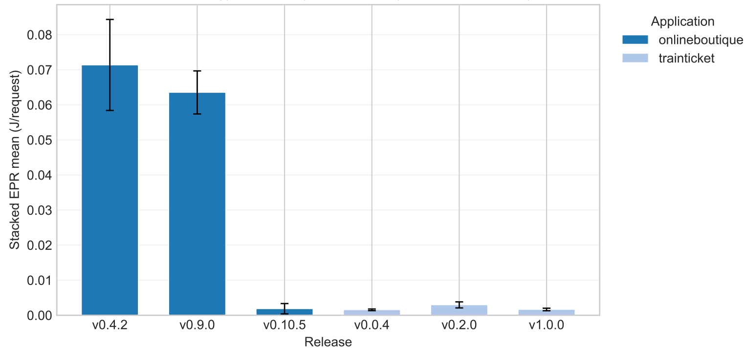
Stacked energy/request by application (workload=medium)
