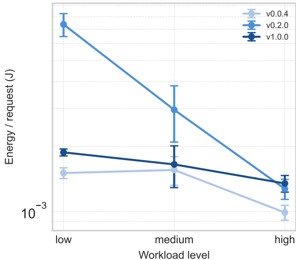
trainticket
