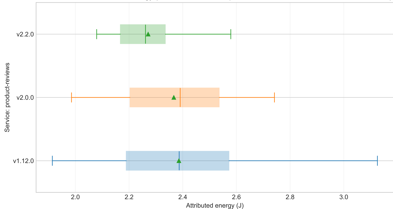
Selected service attributed energy (workstation, service=product-reviews, workload=medium, model=M2)
