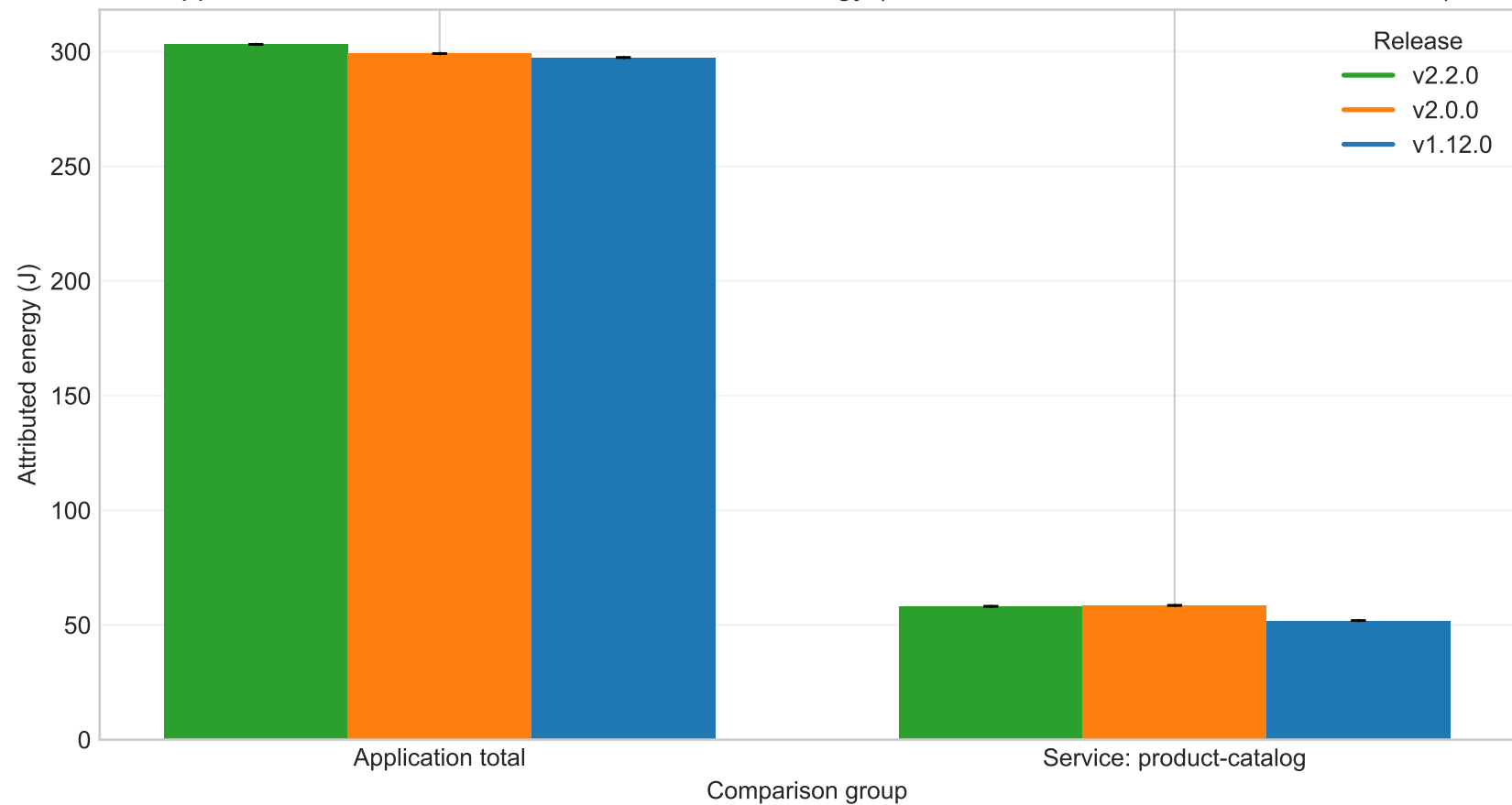
Application total vs selected services attributed energy (workstation, workload=medium, model=M2)
