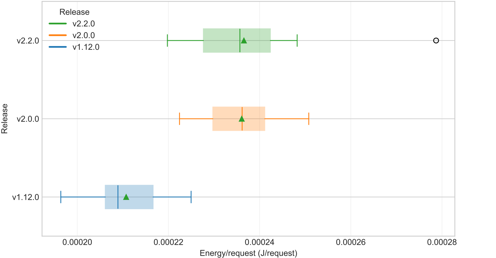
Fixed-util selected service EPR by release (workstation, service=product-catalog, workload=medium, model=M2)
