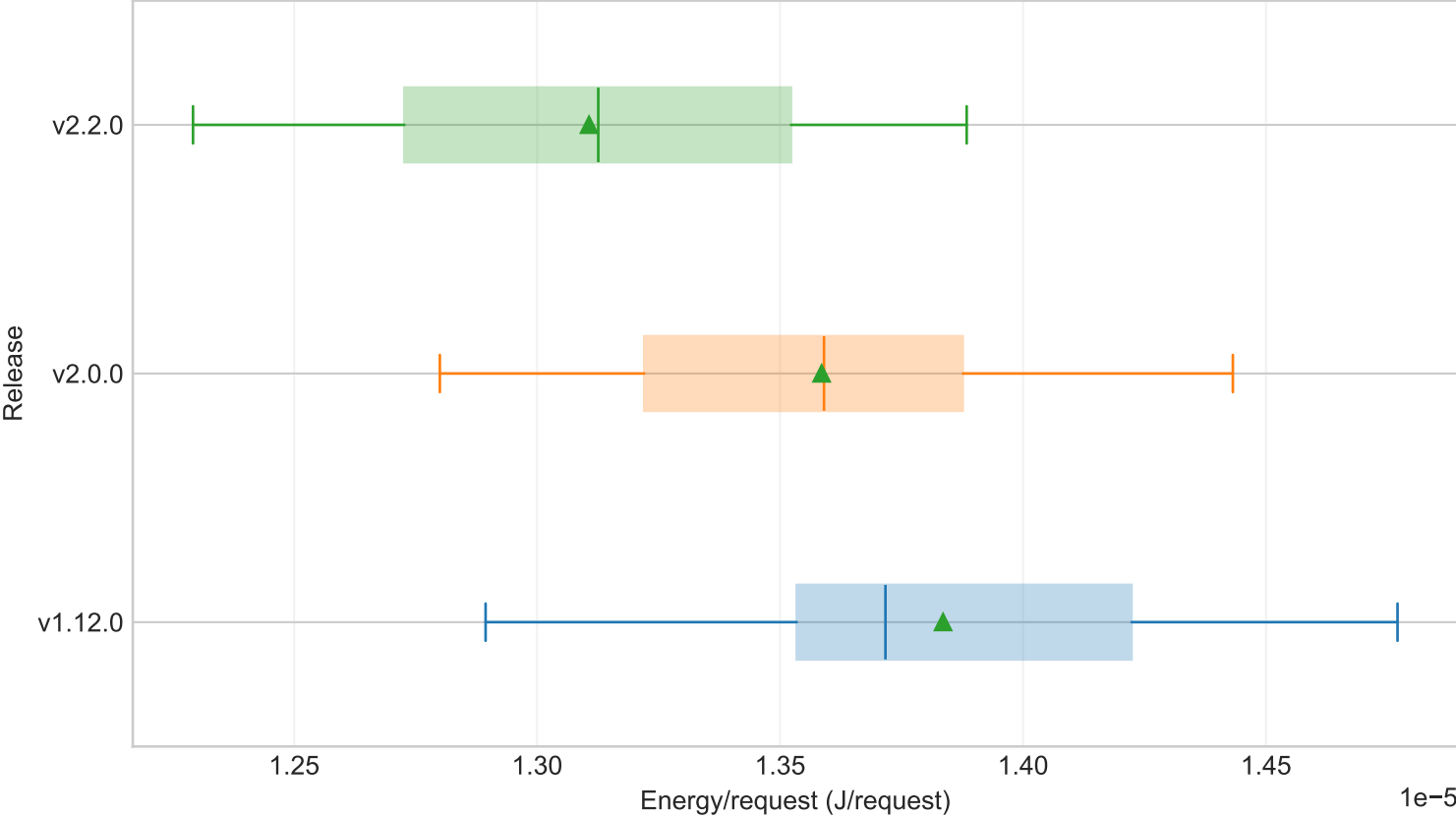
Fixed-util selected service EPR by release (workstation, service=product-reviews, workload=medium, model=M1)
