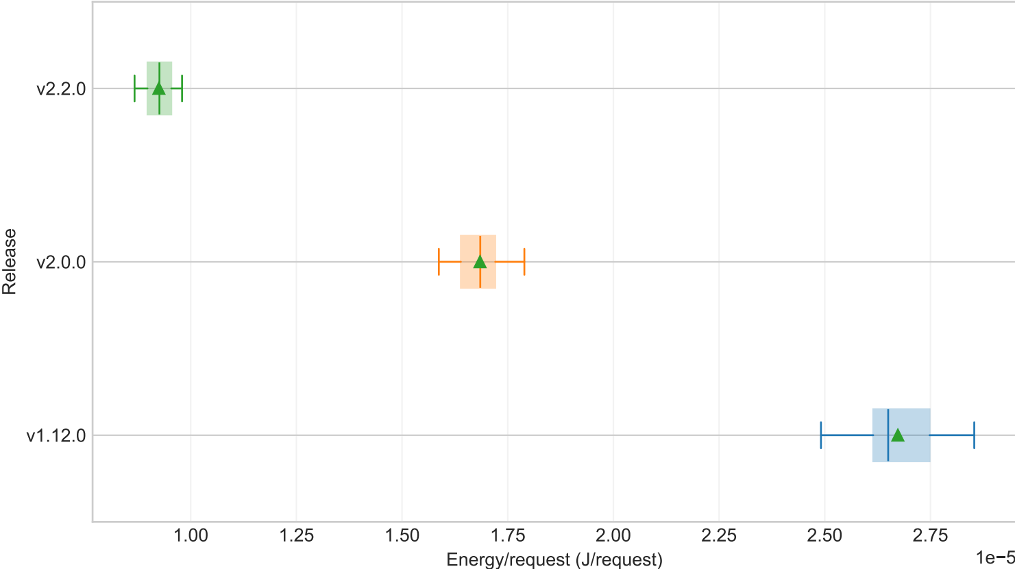
Fixed-util selected service EPR by release (workstation, service=product-reviews, workload=medium, model=M2)
