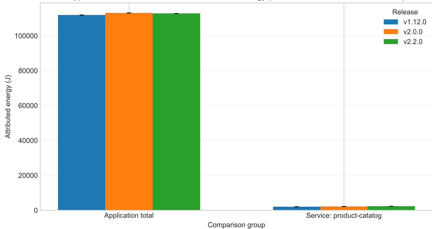
Application total vs selected service attributed energy (ec2, workload=medium, model=M1)
