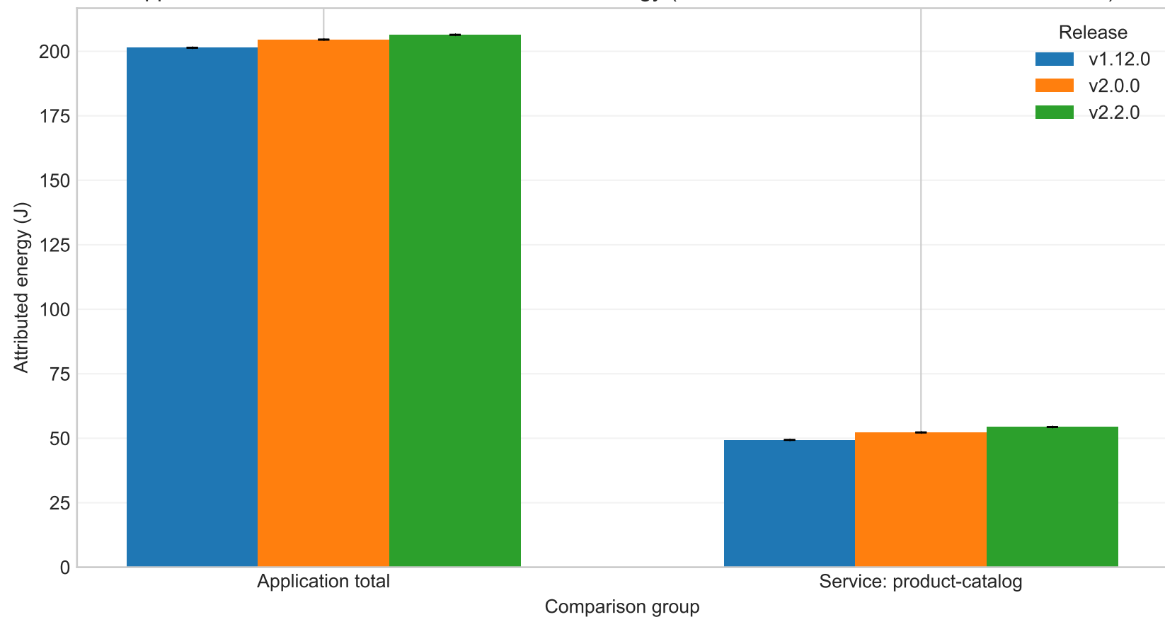
Application total vs selected service attributed energy (workstation, workload=medium, model=M1)
