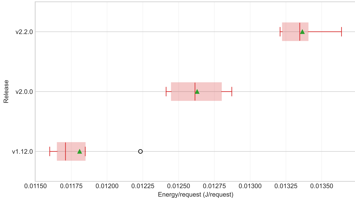
Fixed-util selected service EPR by release (ec2, service=product-catalog, workload=medium, model=M1)
