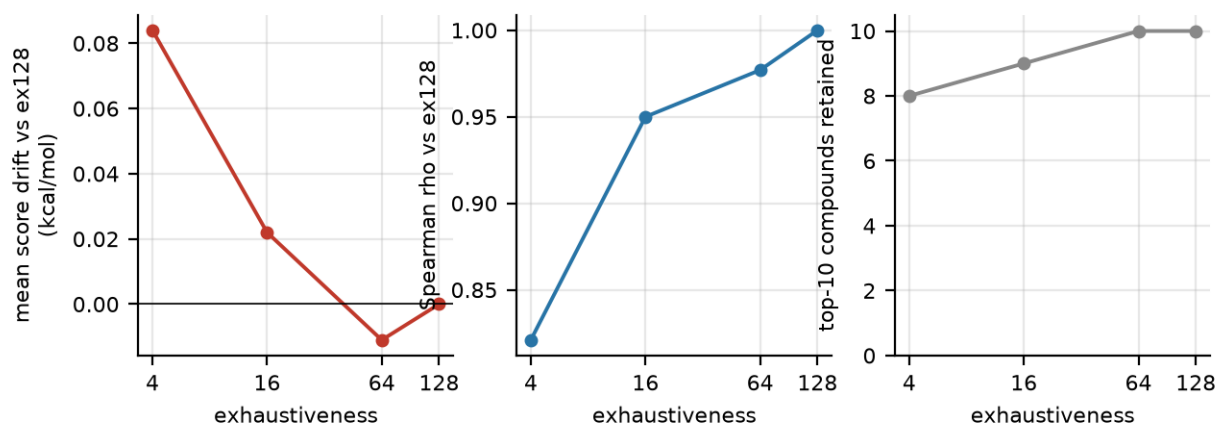
Figure 5. Search effort changes geometry, not ranking. Fifty compounds docked at four exhaustiveness levels with an identical embedding seed, so the only variable is the search. Left, mean score drift against the deepest search. Centre, rank correlation. Right, top-10 compounds retained.
