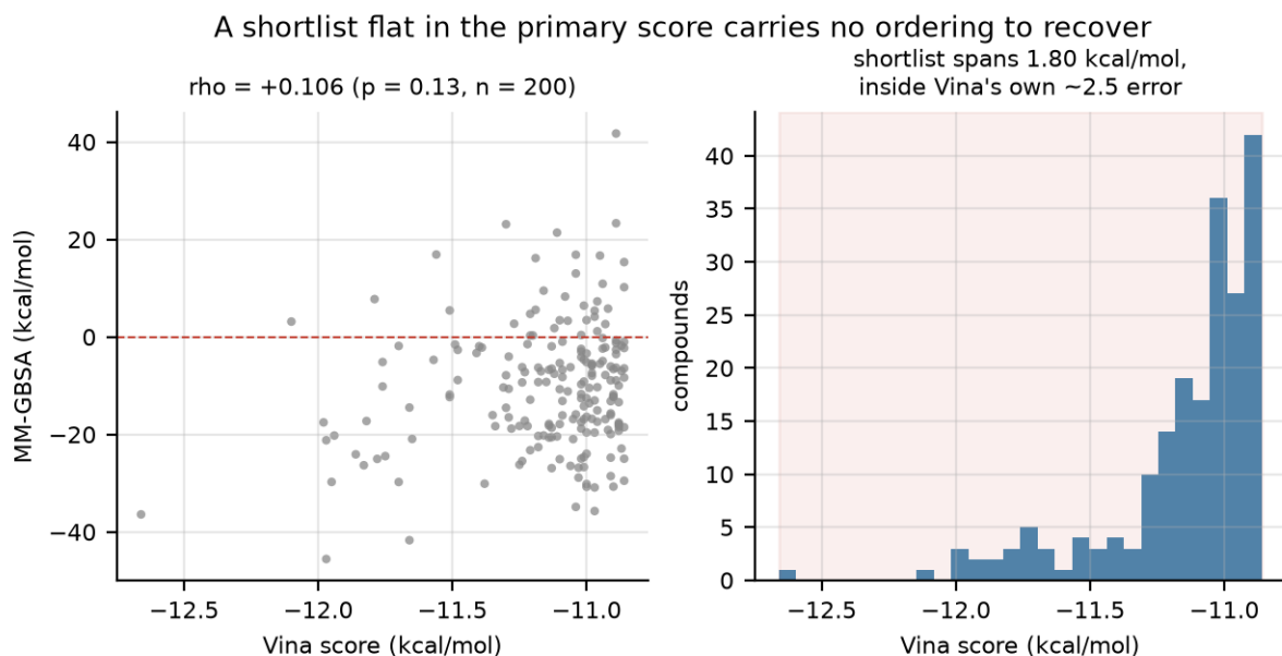
Figure 4. A flat shortlist carries no ordering to recover. Left, MM-GBSA against Vina for all 200 G12V compounds. Right, the Vina score distribution, spanning 1.80 kcal/mol against a documented method error of about 2.5 kcal/mol.
