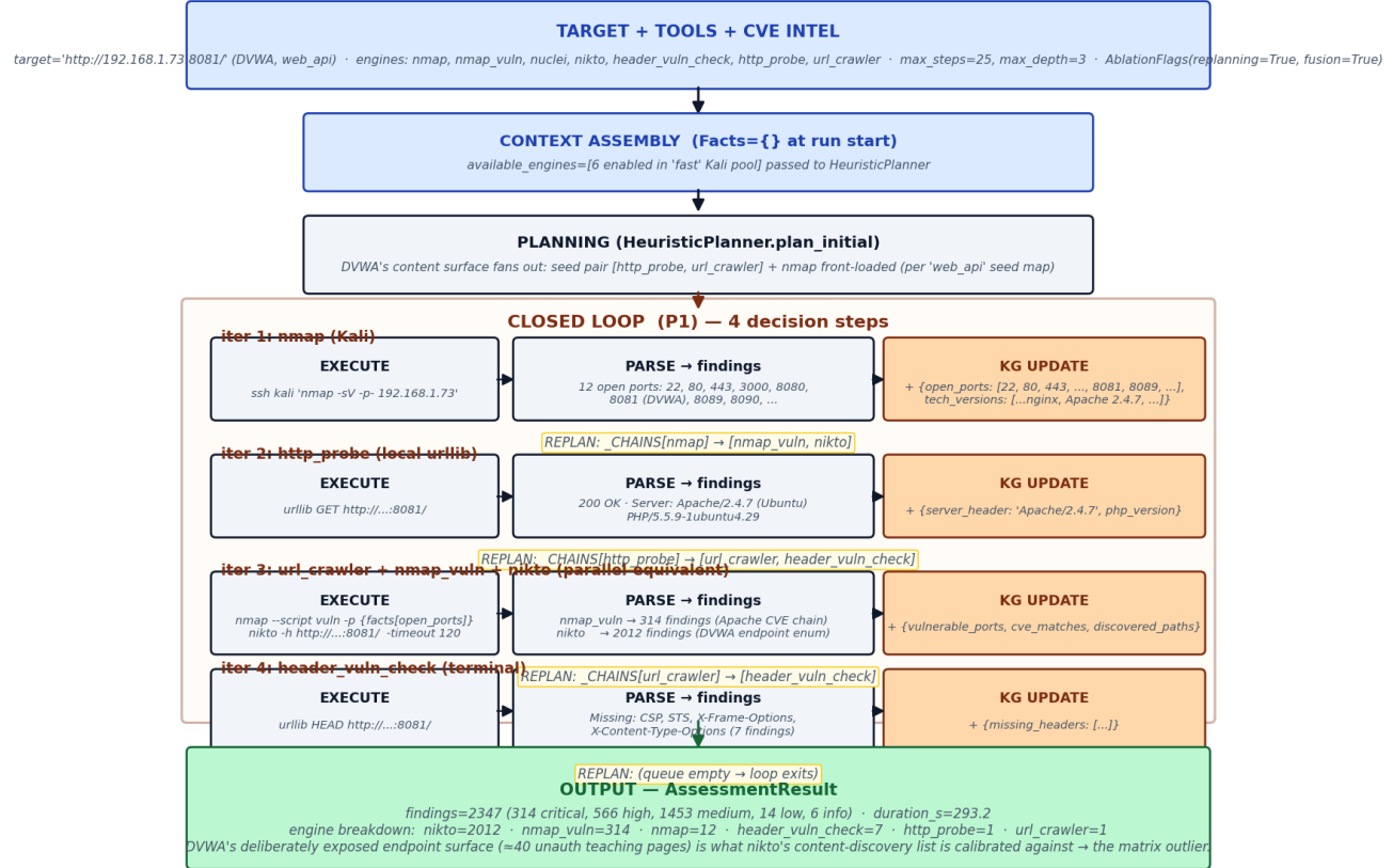
Figure 6 — DVWA full run: scale on a teaching-app surface (2347 findings, the matrix outlier)
