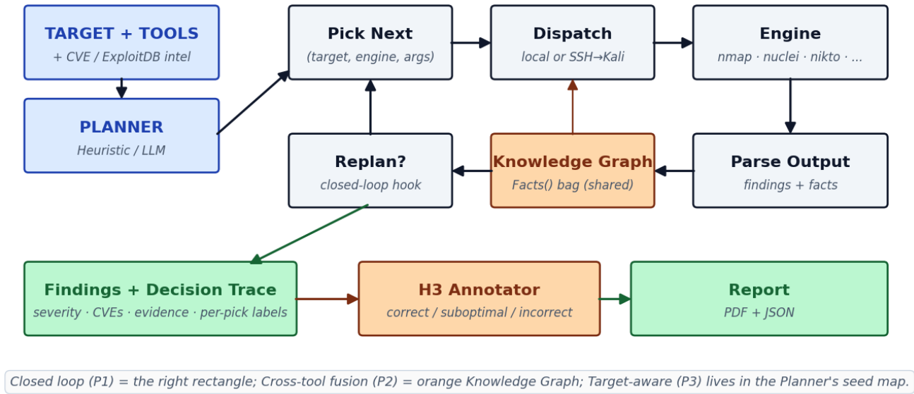
Figure 1: The ReasonChain closed-loop architecture. Blue rectangles are inputs and planner. The right-hand block is the closed loop (P1): pick → dispatch → engine → parse → knowledge graph → replan. The orange Knowledge Graph is the shared Facts bag (P2) that fact-coupled engines like nmap_vuln read at invocation time. Target-aware planning (P3) lives inside the Planner's seed-engine map. Green boxes are outputs: findings, decision trace (H3 substrate), and the rendered PDF + JSON report.
