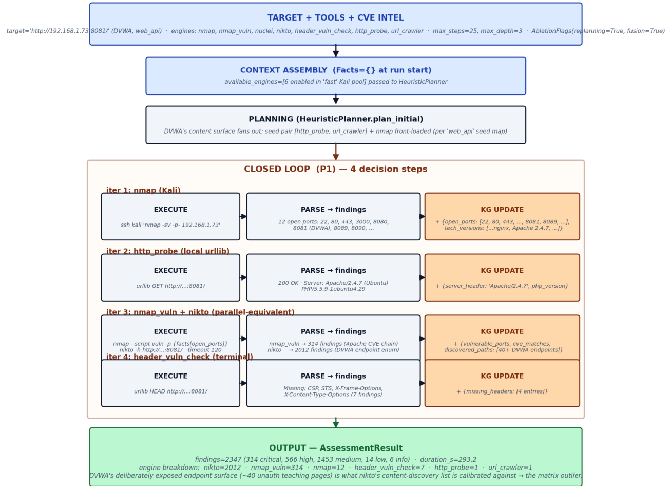
Figure 6: A full-condition run against Damn Vulnerable Web App (DVWA). The matrix outlier: 2347 findings. The same engine chain as Figure 5 runs, but the dominant contributor is nikto's content discovery against DVWA's deliberately exposed unauthenticated teaching surface (2012 of the 2347 findings). nmap_vuln still contributes 314 high-severity findings via the same fact-coupled CVE chain visible in Figure 5. The closed loop completes four decision steps; nikto is queued by the replan after nmap (per the chain map in planner.py:74). Source: per-cell artefact reports/dvwa_live_full_heuristic*.json.
