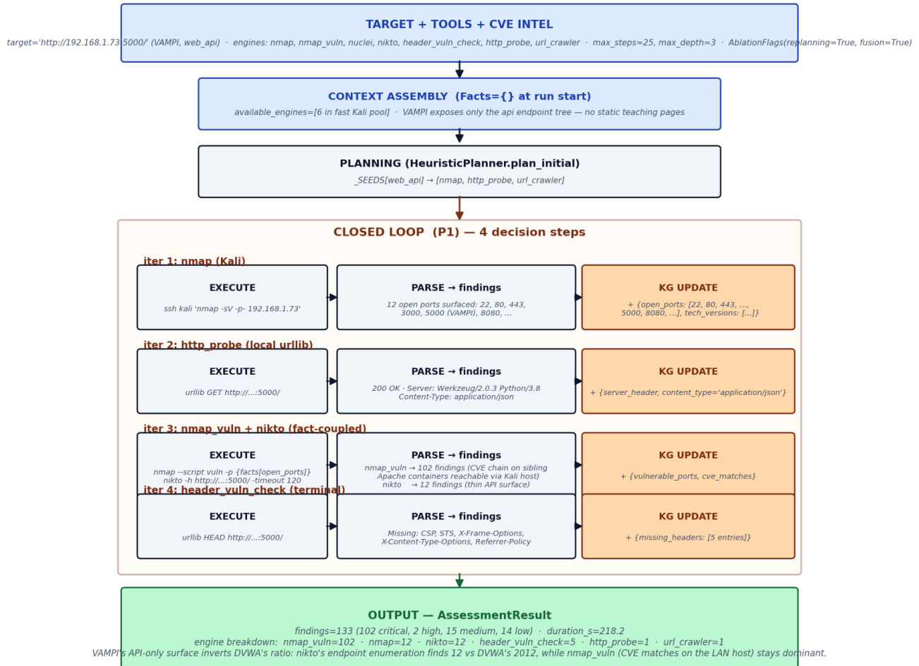
Figure 7 — VAMPI full run: thinner API surface (133 findings, nmap_vuln dominates)
