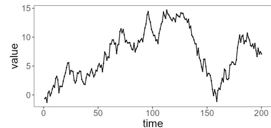
(e) random walk
