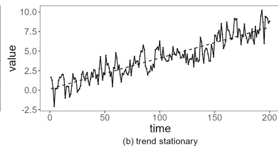
(b) trend stationary
