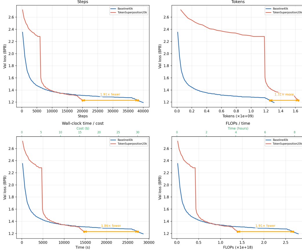
Figure 2: Isoloss curves for validation loss (BPB). X-axes: gradient steps, data tokens processed, wall-clock seconds, and total FLOPs. Y-axis: running minimum validation BPB. The yellow arrow (steps panel) marks the 1.91\times step saving: the baseline requires 38,250 steps to match TST’s final validation loss of 3.41 nats.
