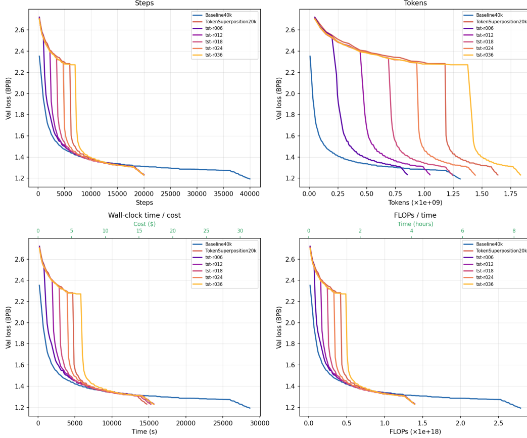
Figure 3: Isoloss curves for validation loss (BPB) for all trained variants: Baseline40k (blue), TokenSuperposition20k ( r=0.30 , red), and the five phase-ratio sweep variants ( r \in \{0.06, 0.12, 0.18, 0.24, 0.36\} , plasma gradient). All TST variants converge to similar final loss, with no meaningful trend across the range of superposition phase lengths.
