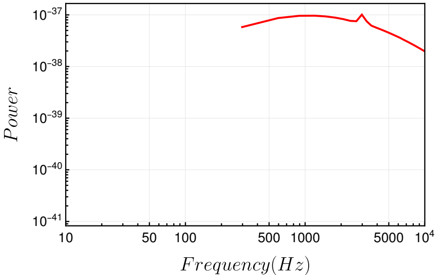
Power Spectrum of GW Signal
