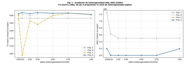
Fig. 1. Heterogeneity gradient, NSL-KDD (2009). F1-macro and ANLL per proposal across seven Dirichlet levels. Proposal A leads B consistently.
