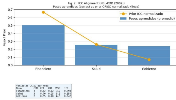
Fig. 2. ICC Alignment, NSL-KDD (2009). Bars: learned weights averaged over 5 reps and 7 levels. Orange line: normalized ICC prior. Financial > Health > Government confirmed.
