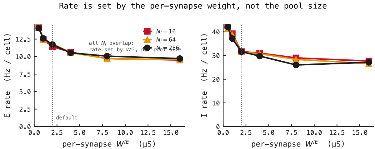
Figure 138: E (left) and I (right) per-cell rate versus the per-synapse weight W^{IE} , one line per pool size N_I . The lines collapse: at any fixed W^{IE} the rate is the same for N_I = 16, 64 , or 256, while it falls steadily with W^{IE} — the logarithmic, saturating dependence of equation (3). The rate is set by the per-synapse kick, not the pool size. Dotted line marks the biophysical default W^{IE} = 2 \mu\text{S} .
