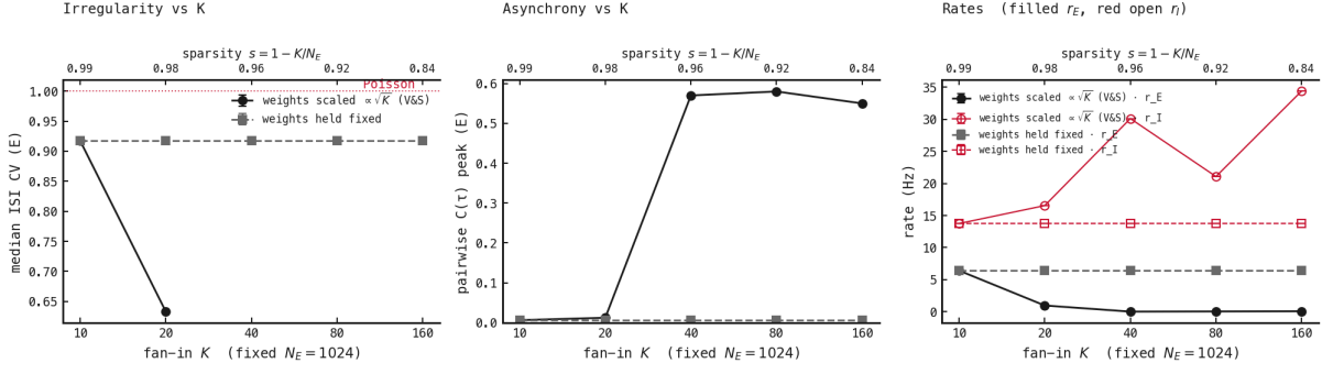
Figure 173: Fan-in K = 10 \rightarrow 160 at fixed N_E = 1024 — equivalently sparsity s = 1 - K/N_E from 0.99 to 0.84 (top axis) — with recurrent weights scaled \propto \sqrt{K} (black, the V&S J/\sqrt{K} rule) versus held fixed (grey); r_I shown in red. \pm 1 SD over three seeds, 3 s trials. What we expect. Strong coupling keeps the O(1) fluctuations, so irregularity survives as K grows; weak coupling loses them ( \propto 1/\sqrt{K} ), so cells regularise . Asynchrony holds in both. What we see. Irregularity: strong stays supra-Poisson (CV 1.2–1.3, easing to 1.11 at K = 160 ); weak decays to \approx 1.0 , the Poisson floor. Asynchrony: both \approx 0.006 throughout. Rates: strong r_E drifts 17.5 \rightarrow 4.9 Hz (the O(1/\sqrt{K}) finite- K correction); weak holds \approx 17 Hz. Do they align? Yes — only J/\sqrt{K} keeps the recurrent irregularity alive as K grows; the gap is the signature. The one mismatch is the strong-coupling rate drift (Next steps); whether the survival is self-generated is settled by Figure 3.
