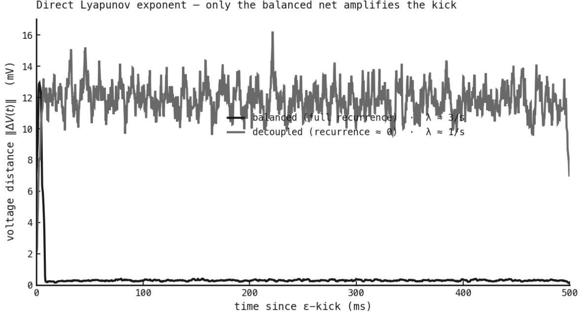
Figure 174: Two clones on identical quenched-DC input, the second kicked by \varepsilon = 0.1 mV at t = 0 ; voltage distance \|\Delta V(t)\| , seed-mean (bold) with a \pm 1 SD band over five seeds, lightly smoothed. What we expect. If chaotic, the kick is amplified — \|\Delta V\| grows exponentially ( \lambda > 0 ) — and with noise-free input that can only be network-generated. The decoupled control should not grow ( \lambda \leq 0 ). What we see. Balanced (black) : \|\Delta V\| rises steeply (fitted rate \lambda \approx +28 s ^{-1} ) then saturates at the attractor size ( \approx 250 mV). Decoupled (grey) : neither amplified nor forgotten — a fixed phase offset, \lambda \approx 0 . Do they align? Yes — \lambda > 0 for the balanced net, \approx 0 for the control: deterministic chaos, self-generated. Caveat: an initial-growth estimate (saturation caps the window), so the sign, not the magnitude, is the result — a renormalised Benettin scheme would pin exact \lambda (Next steps).
