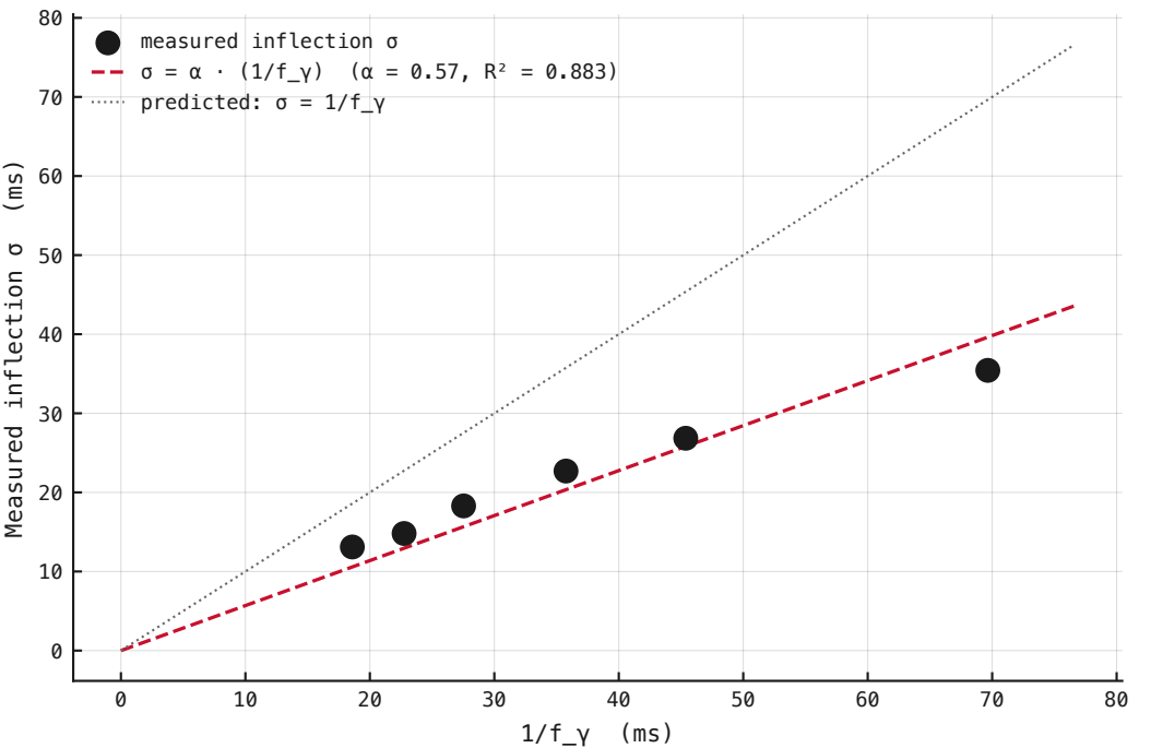
Inflection \sigma tracks 1/f_{\gamma} across \tau_{\text{GABA}}
