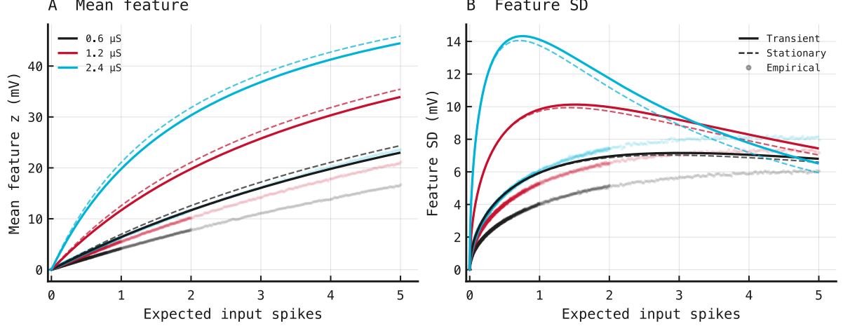
Figure 5: Transient and stationary analytical response moments over input drive. The horizontal axis matches Figure 2: expected input spikes are \lambda \frac{T}{1000} = rx \frac{T}{1000} . Panel A shows mean feature; Panel B shows feature SD. Solid curves are the start-from-rest transient predictions from Equations 18a and 18b; dashed curves are the stationary references from Equations 12a and 18; faint points are the corresponding empirical values from Figure 2. Black, red, and cyan denote probe conductances 0.6, 1.2, and 2.4 \mu\text{S} .
