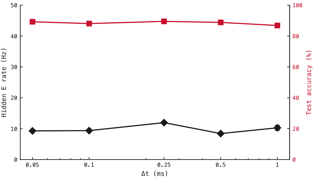
PING \Delta t audit – post-training E rate and accuracy vs integration timestep
