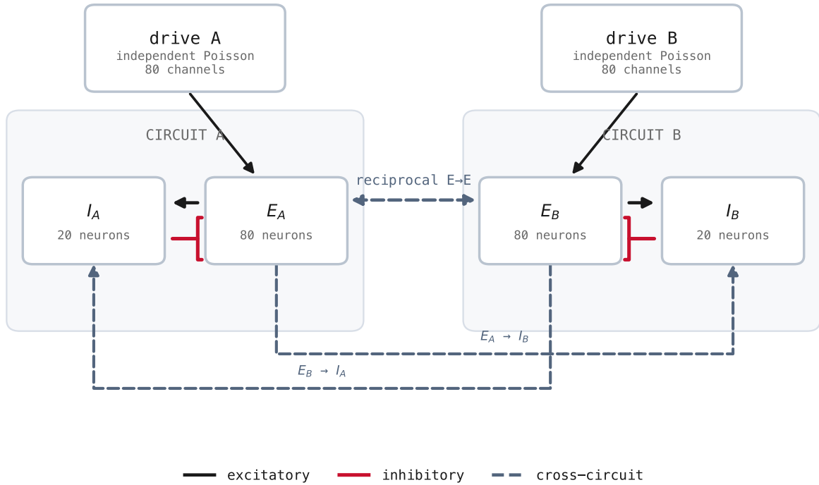
Figure 119: Authored two-circuit network. Each private Poisson input drives a local E-to-I-to-E PING loop. Dashed arrows are the four reciprocal AMPA pathways varied together by K ; red bar-headed arrows are local GABA-A inhibition. The same compiled graph topology is used at every condition.
