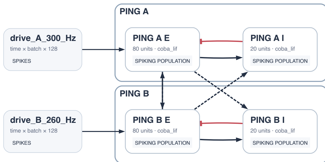
Figure 128: Implemented topology. Networks A and B each contain a local E-to-I-to-E PING loop. Reciprocal projections target E and I populations with independently controlled strengths.
