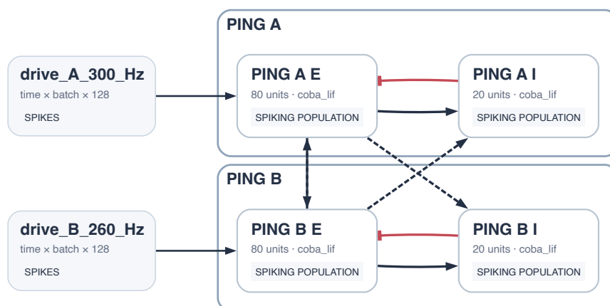
Figure 122: Two matched PING circuits. Long-range excitation targets either E or I with exact fan-in 8.
