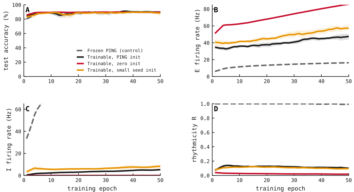
Figure 5: Releasing the loop weights to gradient descent prunes the rhythm within a single epoch, from every initialisation. Per-epoch training metrics with the recurrent weights W^{EI}, W^{IE} made trainable under the Dale’s-law clamp, over 50 epochs on MNIST. Lines are the mean of three seeds (42–44); shading is the across-seed range. Conditions differ only in initialisation of the loop weights: canonical PING values (black), zero (red), and 0.1 \times canonical (amber), against a frozen-PING control (grey, dashed). (A) Test accuracy: all conditions overlap at \approx 84 – 91\% . (B) Mean excitatory firing rate: the trainable conditions rise to \approx 49 – 88 Hz as the loop is dismantled, while the frozen control remains gated near 17 Hz. (C) Mean inhibitory firing rate: the trainable conditions collapse to \approx 0 Hz within a few epochs, while the frozen control’s inhibitory rate rises to \approx 108 Hz as its readout trains. (D) Lobe–trough rhythmicity contrast: the frozen control holds at \approx 1 while every trainable initialisation drains to \approx 0.02 – 0.11 . Source: exp049.
