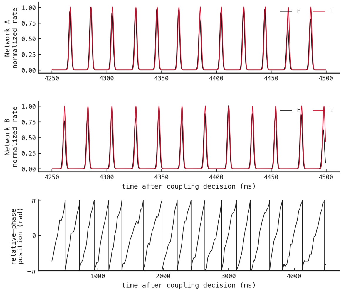
Figure 129: Both uncoupled networks maintain regular PING rhythms, but Network A runs at 50.6 Hz and Network B at 46.6 Hz. Their relative phase therefore circulates, completing 16 slips with phase concentration 0.028.
