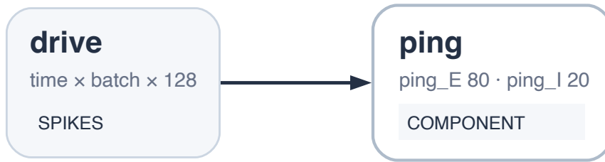
Figure 115: Compiled graph reused at every input condition. A time-by-batch-by-128 spike tensor drives one default PING component with 80 E cells and 20 I cells. Only the input event probability changes across the sweep; the graph and its parameters remain fixed.
