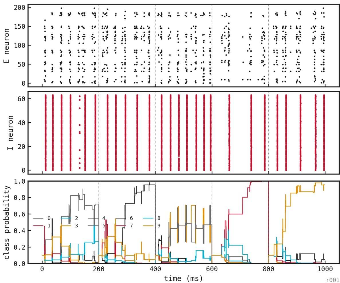
Figure 111: Matched-rate streaming inference with presentation duration equal to the spike-count readout window.
