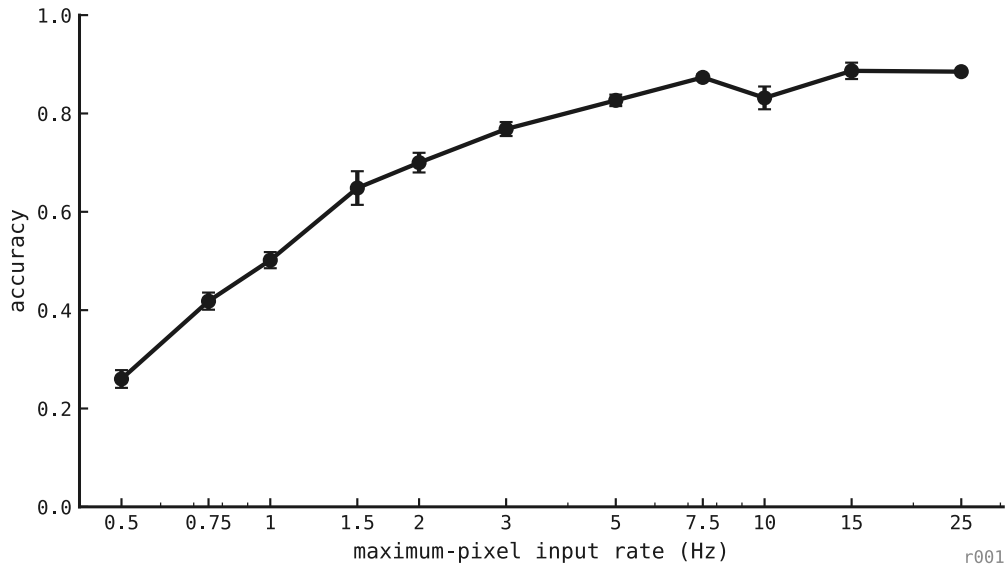
Figure 114: Input-rate psychometric at a fixed 200 ms presentation and spike-count window.
