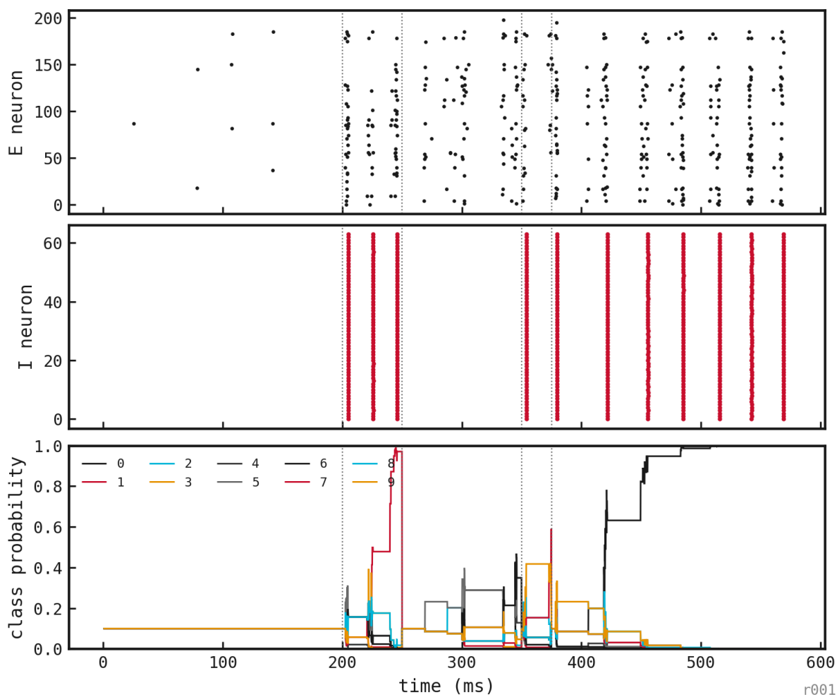
Figure 112: Streaming inference while maximum-pixel input rate and presentation duration vary between digits.
