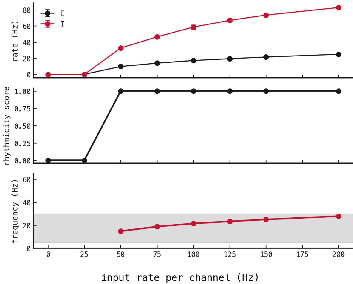
Figure 116: Response of one fixed default PING graph to homogeneous Poisson drive. Top: mean E and I firing rates in hertz, with standard deviations across 5 paired trials. Middle: median lobe-trough rhythmicity contrast R , with error bars showing half the interquartile range; R = 0 is flat and R approaches 1 as periodic structure strengthens. Bottom: median dominant E-population frequency in hertz after subharmonic correction; the grey region marks 5–30 Hz. Rhythmicity switches on abruptly at 50 Hz per channel, while the dominant rhythm increases smoothly from 14.93 Hz.
