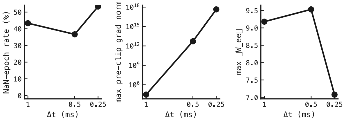
Figure 1: The three stability metrics against \Delta t in ms (coarse \rightarrow fine, left \rightarrow right on each panel): the NaN-epoch rate (%), the peak pre-clip gradient norm (log scale, centre), and the peak E \rightarrow E recurrent-weight norm \|W_{ee}\| (right). What we expect if the plan’s hypothesis holds: all three fall as \Delta t shrinks, the NaN-epoch rate toward zero and the gradient and weight norms toward bounded values. What we see refutes it. Not one of the three metrics improves as \Delta t shrinks. The NaN-epoch rate does not fall toward zero: 13 of 30 epochs diverge at \Delta t = 1.0 , 11 at 0.5, and 16 at 0.25 (flat-to-worse, not a descent). The peak pre-clip gradient norm moves the wrong way and violently, climbing from \approx 10^4 at \Delta t = 1.0 to \approx 10^{18} at \Delta t = 0.25 , roughly 14 orders of magnitude the wrong way. Only the excitatory-to-excitatory recurrent-weight norm \|W_{ee}\| stays in one range (7.1–9.5), so this is not a runaway-weight story.
