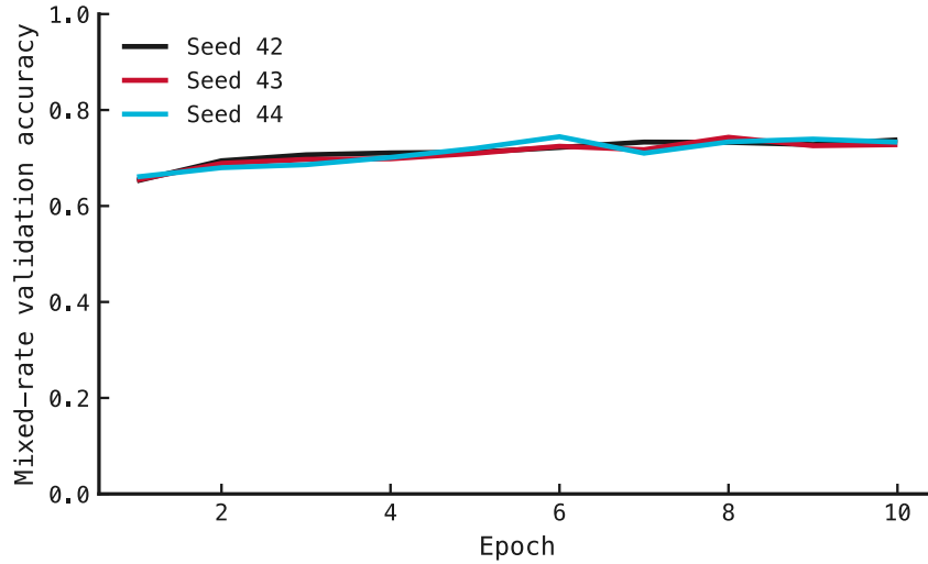
Figure 125: Mixed-rate validation accuracy across training. The horizontal axis is epoch and the vertical axis is validation accuracy. Each curve is one independently trained nonlinear decoder, and every epoch uses fresh direct feature simulations. All three decoders improve before checkpoint selection.
