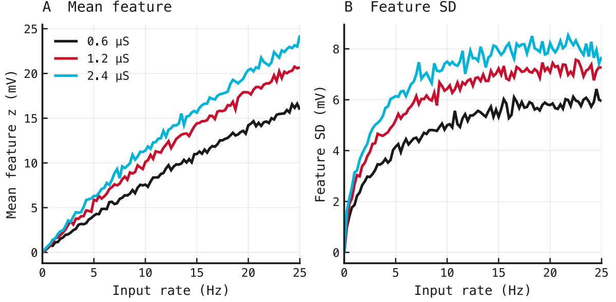
Figure 128: Empirical finite-window response of a fully active pixel over the input-rate grid. Both horizontal axes show input rate in spikes/s. Panel A shows mean feature in mV; Panel B shows feature SD in mV. Each coloured curve contains 101 rate conditions. At every rate, the plotted mean or SD summarizes 512 independently simulated presentations; the figure does not display those individual presentations as points. Black, red, and cyan denote 0.6, 1.2, 2.4 \mu\text{S} conductance increments. Mean response rises with rate, while variability reaches a broad maximum or plateau.
