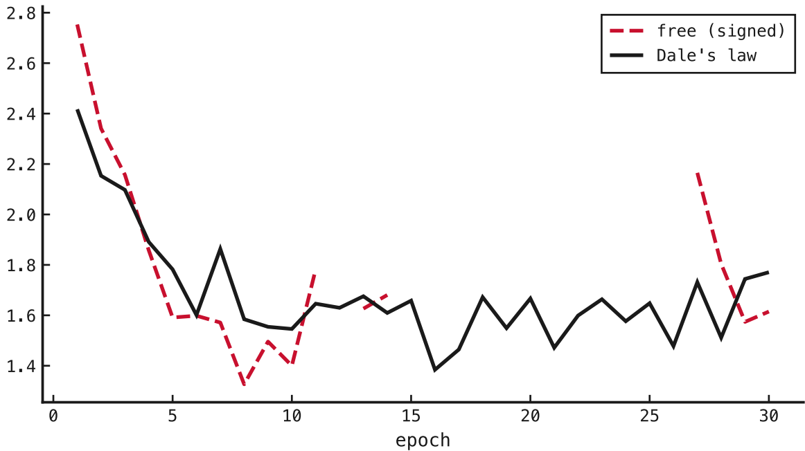
test cross-entropy loss
