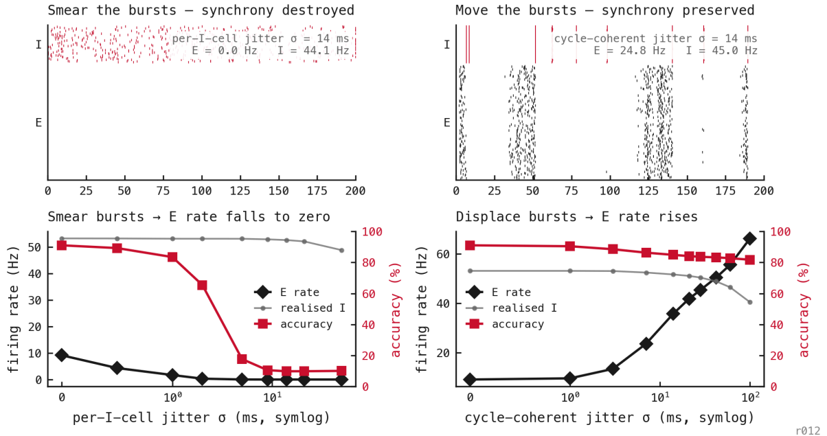
Figure 10: Two inhibitory-jitter manipulations at the same magnitude that hold the mean inhibitory rate fixed drive the excitatory rate in opposite directions, isolating timing from level. The trained PING inhibitory spike train is perturbed at inference while the mean per-cell inhibitory rate is held constant. Both arms use the same jitter magnitude, \sigma = 14 ms — only the kind of jitter differs. Top: single-trial rasters (E black, I red). Bottom: mean excitatory rate (black) and accuracy (red) versus jitter magnitude \sigma , with the realised mean inhibitory rate overlaid (grey). Left: per-cell jitter smears each burst into a continuous shunt; the excitatory rate falls to \approx 0 Hz (inhibitory rate \approx 53 Hz) and accuracy falls to chance. Right: cycle-coherent jitter displaces whole bursts while preserving within-burst synchrony; the excitatory rate rises from \approx 9 to \approx 36 Hz (inhibitory rate \approx 52 Hz, matched to the left arm) and accuracy holds high. Both arms are read where the realised inhibitory rate is matched to within a few percent; at larger \sigma the cycle-coherent excitatory rate climbs further, but the finite trial window truncates the most-displaced bursts and realised inhibition falls, so the strict comparison is anchored here. Identical mean inhibition, opposite excitatory outcome: the gate is the phase structure of inhibition, not its level. Source: exp042.
