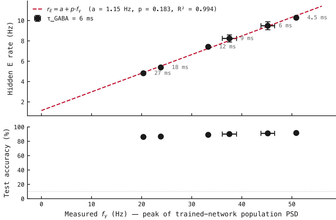
Figure 6: The post-training excitatory firing rate is an affine function of the gamma frequency. Networks were trained from scratch at each of six values of the GABA decay constant \tau_{\text{GABA}} \in \{4.5, 6, 9, 12, 18, 27\} ms, which sets the realised gamma frequency f_\gamma (§5.4). Top: mean post-training excitatory firing rate against measured f_\gamma ; markers are per-condition means over three seeds, with error bars ( \pm SD) on both axes. The linear fit r_E = 1.15 + 0.183f_\gamma passes through every error bar ( R^2 = 0.994 ). Bottom: test accuracy over the same range, flat at 86–92%, so the frequency-set rate constraint does not trade against accuracy. Source: exp041.
