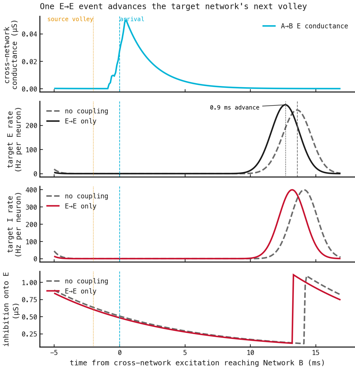
Figure 6: The first measurable E-to-E correction after coupling begins. Time zero is the arrival of excitation from Network A at Network B. Dashed grey traces show the no-coupling branch from the same saved state. Solid traces show the E-to-E-only branch.
