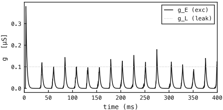
PING · I-neuron conductances (cell 1)
