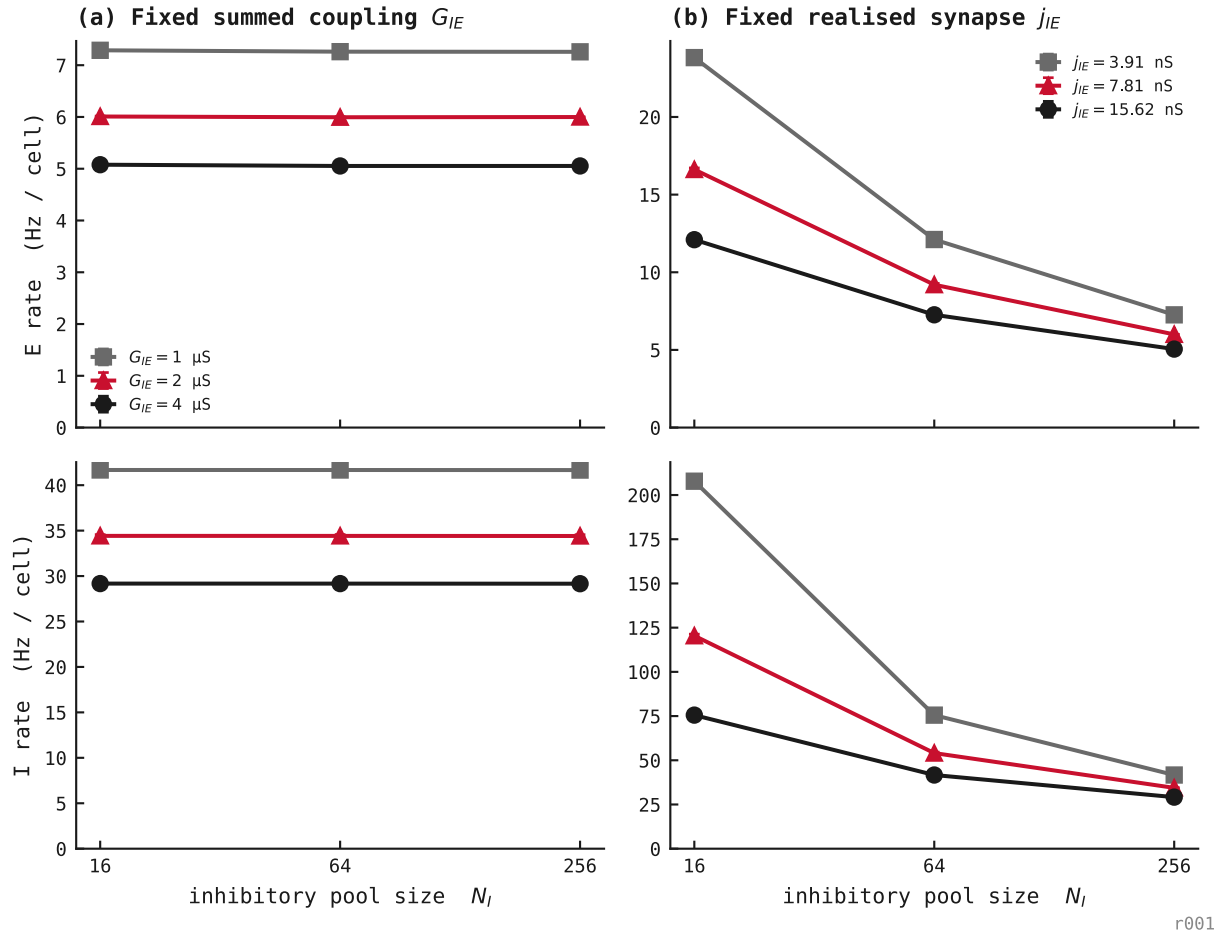
Figure 83: Excitatory and inhibitory firing rates across inhibitory-pool size under two I→E scaling controls. Top: excitatory-cell rate in Hz per cell. Bottom: inhibitory-cell rate in Hz per cell. (a) Holding the expected summed I→E coupling G_{IE} fixed makes the realised synapse j_{IE} = \frac{G_{IE}}{N_I} shrink as the pool grows. (b) Holding j_{IE} fixed makes summed coupling grow with N_I . Each curve is one coupling level; markers are means and error bars \pm 1 standard deviation (SD) over 3 seeds, with 8 trials per seed. The controls coincide at the reference pool N_I = 256 . Rates are invariant to pool size only under inverse scaling of individual synapses.
