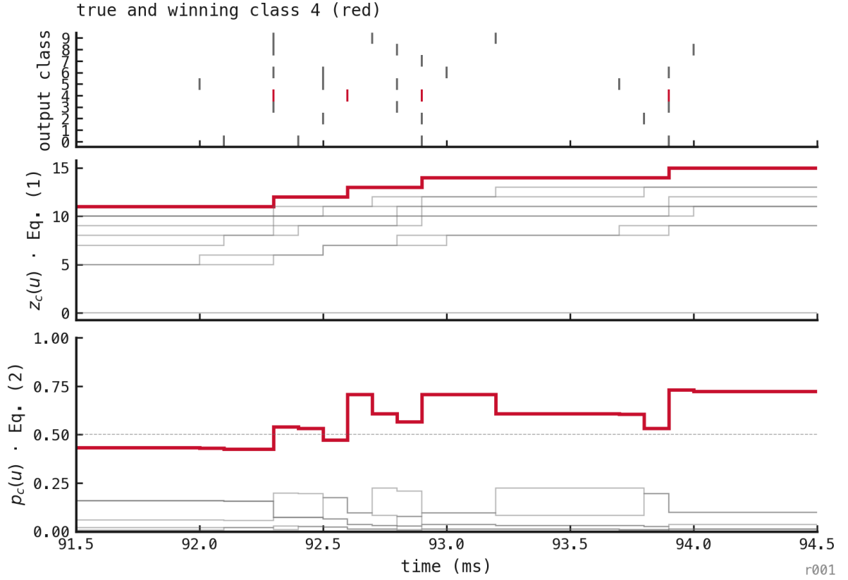
Figure 112: A post-hoc enlargement of 91.5–94.5 ms in the same trial. Each spike increments one cumulative count. Softmax normalization can lower another class’s displayed share even when its count does not change.
