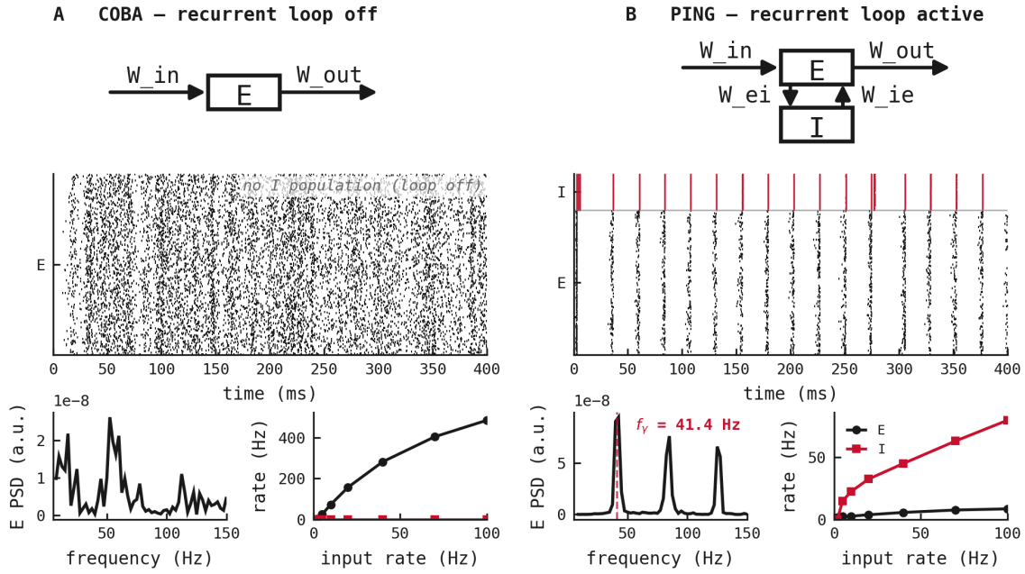
Figure 35: The architecture and its behaviour, off and on, on the same network. Each column carries its schematic on top — A COBA (input→ E →output, no I population) and B PING (the same plus the recurrent E \leftrightarrow I loop, W_{ei} down and W_{ie} up) — directly above the plots it produces. Below each schematic is one combined raster ( E black in the lower portion, I red in the upper portion — same axes, no gap) above a bottom row pairing the Welch PSD of the population-mean E trace with the free-running f - I curve (mean per-cell rate vs input rate, E black / I red; each column has its own y-axis — COBA runs to its \approx 400+ Hz ceiling, PING is on a smaller scale so its loop-clamped E and climbing I are legible). Rasters and spectra are on uniform Poisson input (400 ms) at per-condition rates (COBA 5 Hz, PING 45 Hz — see Methods); the f - I curves sweep that drive on the untrained network. All runs are at \Delta t = 0.1 ms. A — COBA ( ei -strength 0, loop off): asynchronous E firing, no I activity, no recurrent gamma peak, and an E f - I curve that climbs steeply with input rate and saturates toward the refractory ceiling. B — PING ( ei -strength 1.5, loop on): the I population fires a synchronous burst once per cycle and the E raster breaks into vertical bands (the I volley trails each E volley by the AMPA delay); the PSD carries a clean gamma peak (dashed red line; f_\gamma measured from this raster’s E -population PSD, marked on the plot); and its f - I shows the E rate held to single digits across the whole sweep (note the much smaller y-axis than COBA’s) while inhibition climbs — the loop’s dynamic-range compression. The single E \rightarrow I \rightarrow E loop is the only change: it converts asynchronous firing into a gamma rhythm and clamps the E rate.
