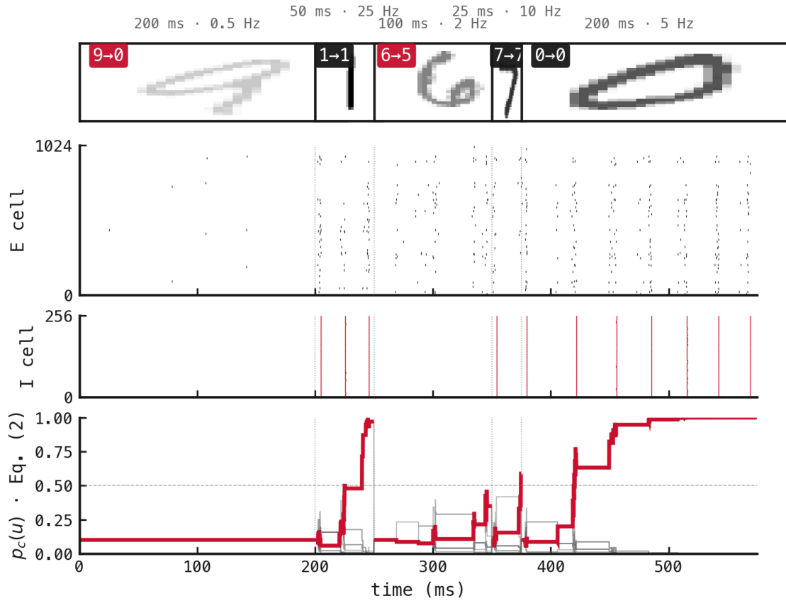
Figure 113: A five-digit stream classified by the native output-LIF spike-count readout. Counts reset at each boundary; hidden PING state continues. Thumbnail opacity increases with input rate, and badges show the true and predicted labels.
