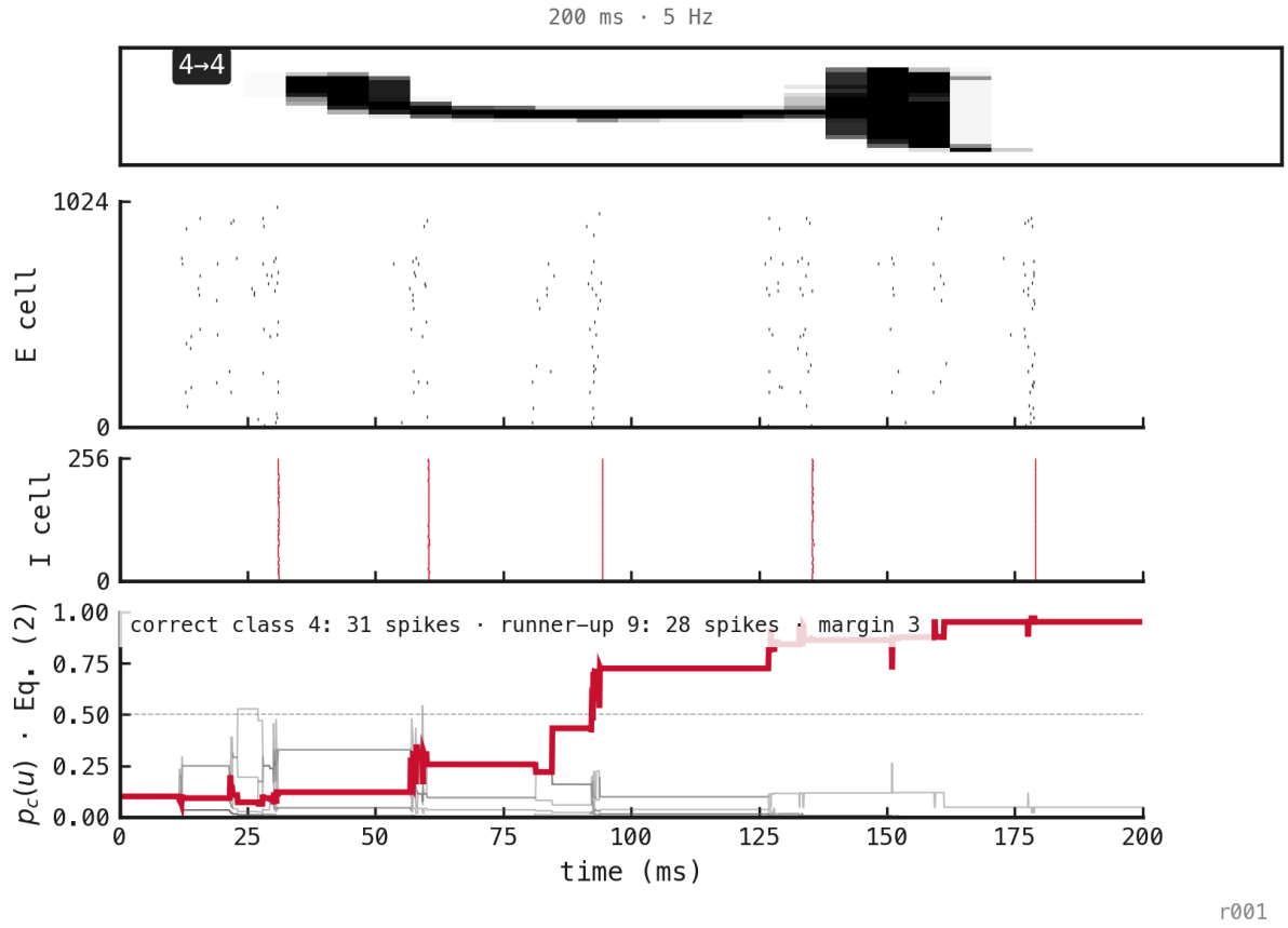
Figure 111: A correctly classified 200 ms presentation at 5 Hz, selected as the first success in a pre-existing matched stream. The figure explains the readout; it does not estimate accuracy. Red marks the true and winning class.
