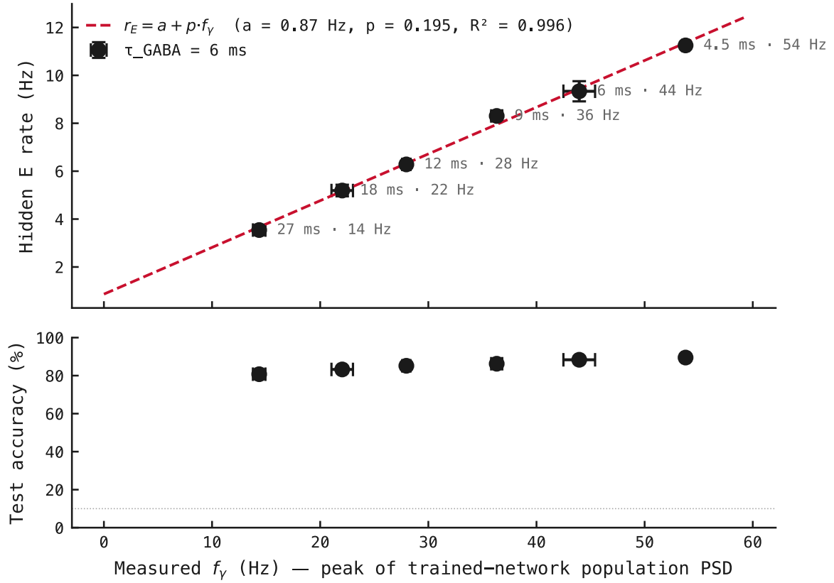
Figure 6: The post-training excitatory firing rate is an affine function of the gamma frequency. Networks were trained from scratch at each of six values of the GABA decay constant \tau_{\text{GABA}} \in \{4.5, 6, 9, 12, 18, 27\} ms, which sets the realised gamma frequency f_\gamma (§5.4). Top: mean post-training excitatory firing rate against measured f_\gamma ; markers are per-condition means over three seeds, with error bars ( \pm SD) on both axes. The linear fit r_E = 0.76 + 0.216f_\gamma passes through every error bar ( R^2 = 0.997 ). Bottom: test accuracy over the same range, flat at 81–89%, so the frequency-set rate constraint does not trade against accuracy. Source: exp041.
