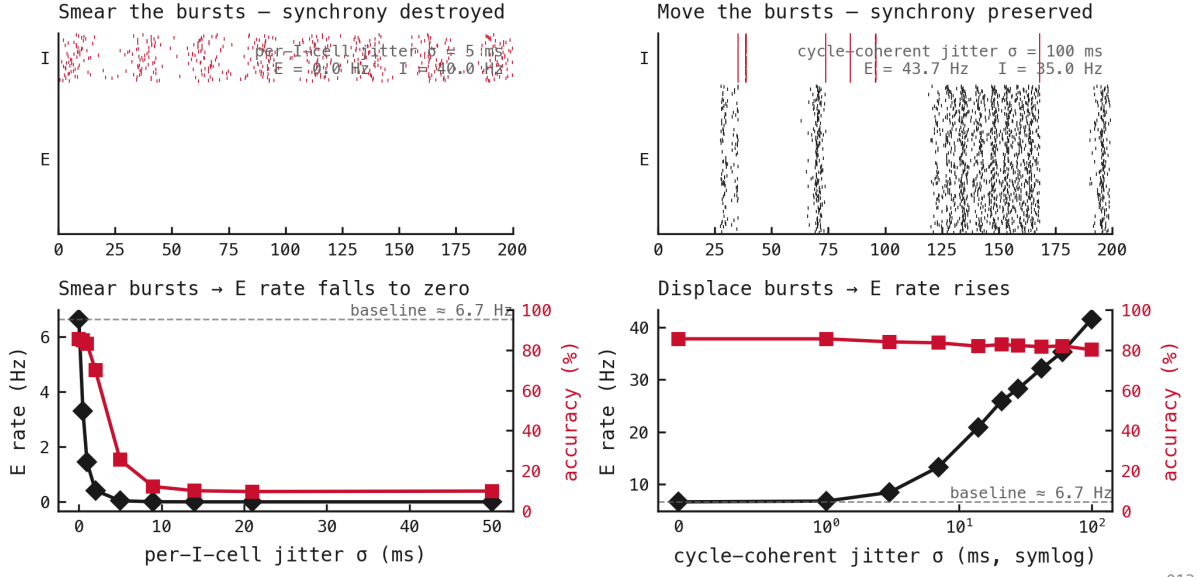
Figure 10: Two inhibitory-jitter manipulations that hold the mean inhibitory rate fixed drive the excitatory rate in opposite directions, isolating timing from level. The trained PING inhibitory spike train is perturbed at inference while the mean per-cell inhibitory rate is held constant. Top: single-trial rasters (E black, I red). Bottom: mean excitatory rate (black) and accuracy (red) versus jitter magnitude \sigma . Left: per-cell jitter ( \sigma = 5 ms) smears each burst into a continuous shunt; the excitatory rate falls to \approx 0 Hz (inhibitory rate \approx 40 Hz) and accuracy falls to chance. Right: cycle-coherent jitter ( \sigma = 100 ms) displaces whole bursts while preserving within-burst synchrony; the excitatory rate rises from \approx 8 toward \approx 50 Hz (inhibitory rate \approx 35 Hz) and accuracy holds near 80%. Identical mean inhibition, opposite excitatory outcome: the gate is the phase structure of inhibition, not its level. Source: exp042.
