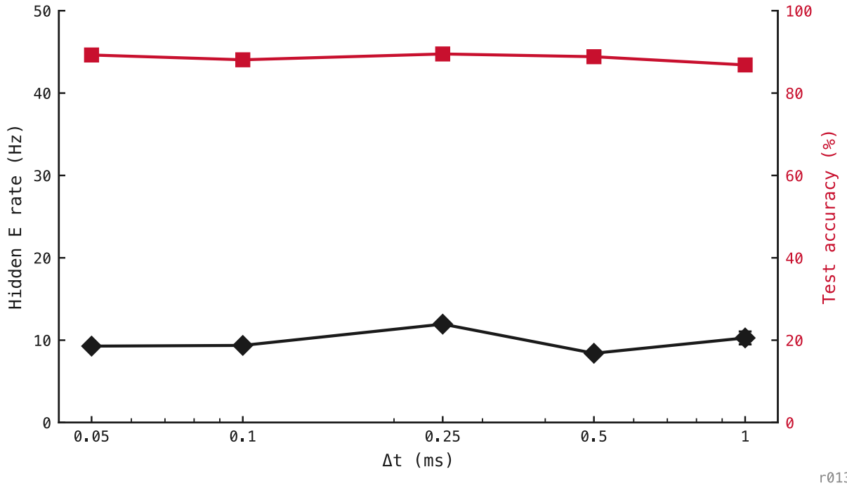
Figure 11: The firing-rate reduction is a physical-time property, invariant to the integration timestep over a twentyfold range. The network was trained and evaluated at matched integration timestep \Delta t for each value across [0.05, 1.0] ms (logarithmic abscissa). Left ordinate (black diamonds): post-training mean excitatory rate, confined to an 8.4–12 Hz band and non-monotonic in \Delta t , so finer stepping does not buy a lower rate. Right ordinate (red squares): test accuracy, flat within 2.7 pp (86.8–89.5%). Because both training and inference use the same \Delta t at each point, the figure tests invariance of the training-plus-inference pipeline, not the generalisation of one trained network to a varied inference step. Source: exp044.
