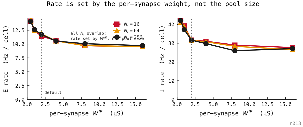
Figure 8: The firing-rate reduction is set by the strength of each inhibitory synapse, not by the size of the inhibitory pool. Per-cell firing rates as a function of the per-synapse I→E weight W^{IE} (0.5–16 \mu\text{S} ), swept independently at three inhibitory pool sizes N_I \in \{16, 64, 256\} . Left: excitatory rate, falling from \approx 14 Hz at W^{IE} = 0.5 \mu\text{S} to \approx 9.6 Hz at W^{IE} = 16 \mu\text{S} . Right: inhibitory rate, falling from \approx 42 to \approx 27 Hz. In both panels the three pool-size curves are superimposed, so the rate is governed by the per-synapse inhibitory gain rather than by interneuron count. The dashed vertical line marks the canonical W^{IE} = 2 \mu\text{S} . Source: exp047.
