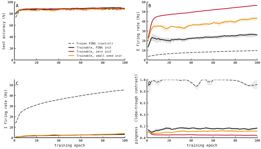
Figure 5: Releasing the loop weights to gradient descent prunes the rhythm within a single epoch, from every initialisation. Per-epoch training metrics with the recurrent weights W^{EI}, W^{IE} made trainable under the Dale’s-law clamp, over 100 epochs on MNIST. Lines are the mean of three seeds (42–44); shading is the across-seed range. Conditions differ only in initialisation of the loop weights: canonical PING values (black), zero (red), and 0.1 \times canonical (amber), against a frozen-PING control (grey, dashed). (A) Test accuracy: all conditions overlap at \approx 88 – 90\% . (B) Mean excitatory firing rate: the trainable conditions rise to \approx 25 – 55 Hz as the loop is dismantled, while the frozen control remains gated near 8 Hz. (C) Mean inhibitory firing rate: the trainable conditions collapse to \approx 0 Hz within a few epochs, while the frozen control’s inhibitory rate rises to \approx 45 Hz as its readout trains. (D) Lobe–trough rhythmicity contrast: the frozen control holds at \approx 0.9 while every trainable initialisation drains to \approx 0.04 – 0.18 . Source: exp049.
