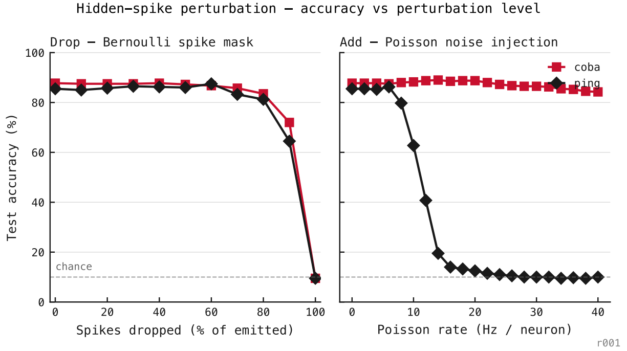
Figure 9: The gating is robust to spike deletion but fragile to spike addition — the expected signature of a phase-based code. A trained PING network is perturbed at inference (no retraining); accuracy is plotted against perturbation level. Left: deletion of a random fraction of emitted spikes. PING retains \approx 82\% accuracy — essentially its unperturbed value — through 80% deletion, degrading only as the network approaches silence. Right: addition of Poisson spikes, expressed as a fraction of each population’s baseline rate. PING accuracy falls sharply, reaching chance between \approx 15 and 65% added noise, because off-phase spikes drive the inhibitory pool at arbitrary phase and dissolve the rhythm. COBA (red), having no rhythm to protect, shows the mirror-image asymmetry: tolerant to addition, intolerant to deletion. Source: exp037.
