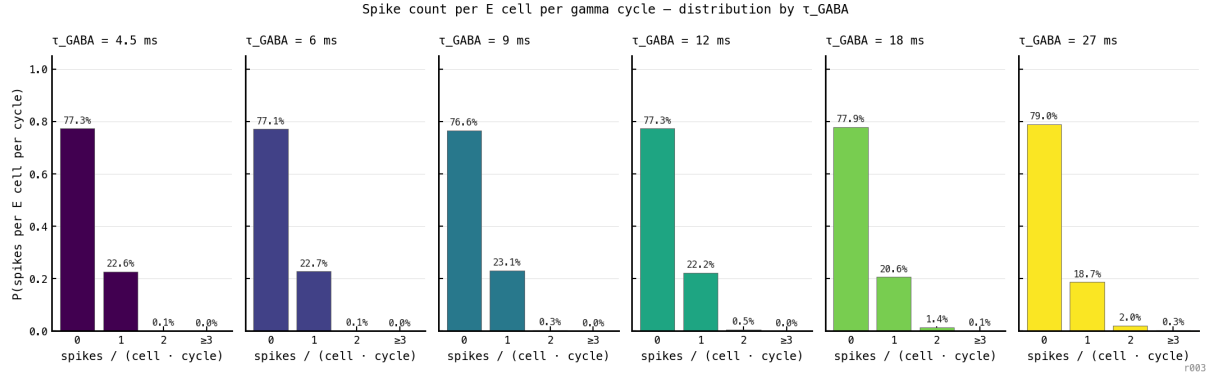
Figure 7: The affine rate law follows from a near-binary per-cycle firing statistic: each excitatory cell contributes at most one spike per gamma cycle. Excitatory spikes were resolved into (cell, cycle) pairs by assigning each spike to the gamma cycle inferred from peaks of the population inhibitory-burst rate (§5.5). Each panel shows the distribution of spikes per pair — 0, 1, 2, or \geq 3 — at one value of \tau_{\text{GABA}} . Across the sweep, P(0) \approx 77\% , P(1) \approx 22\% , and the multi-spike fraction ( \geq 2 ) stays below \approx 3\% ; pooled over all conditions, 99.45% of pairs contain at most one spike. Source: exp046.
