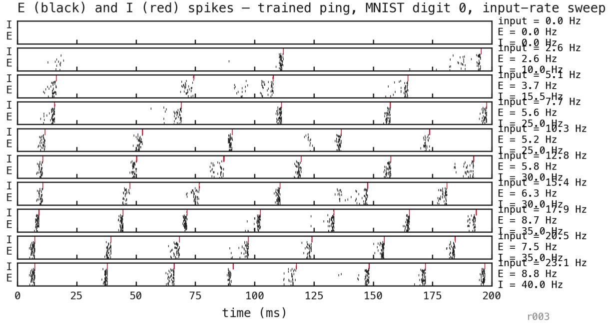
Figure 58: Trained PING (the exp025 baseline) replayed on MNIST digit 0 across ten input-rate values from 0 up to \approx 23 Hz; each panel is one rate, E spikes (black) above I spikes (red), labelled with the input rate and resulting per-cell E and I rates. Reading down the stack: at low drive the network is silent (E and I both 0); past a recruitment threshold ( \approx 8 Hz input) the I-loop catches — I jumps from 0 to \approx 10 Hz and gamma bands appear; above that the E rate stays pinned near 4–5 Hz while I climbs toward \approx 25 Hz, and the cycle period barely moves with further drive. (The faint clustering in the just-engaged panels, where I is still 0, is feedforward input structure, not PING — see Discussion.)
