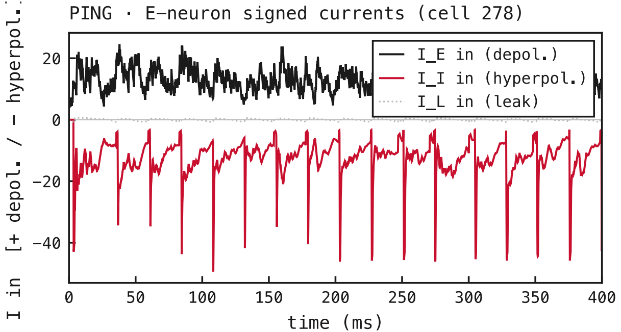
Figure 54: The load-bearing panel. Signed currents into the E cell, PING mode. The excitatory current I_E^{\text{in}} = -g_E(V - E_E) (black) is depolarising; the inhibitory current I_I^{\text{in}} = -g_I(V - E_I) (red) is negative (hyperpolarising) even though g_I is positive (Figure 3b) — the minus sign comes entirely from the driving force ( V - E_I > 0 whenever V sits above E_i = -80 mV). The COBA principle made literal: the sign lives in the driving force, never in the conductance . The sharp negative pulses are the per-cycle inhibitory kicks that gate the rhythm.
