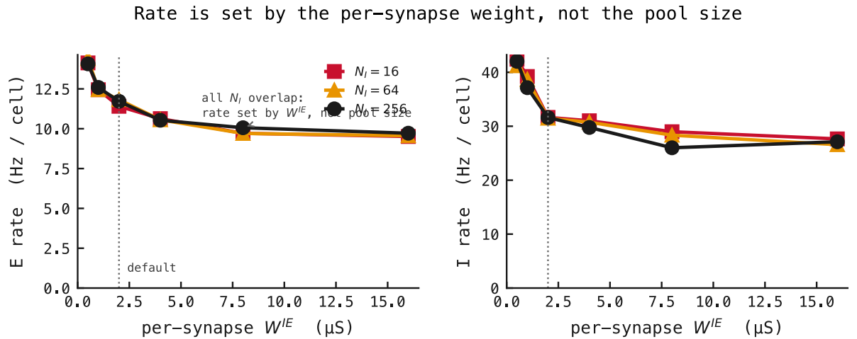
Figure 138: E (left) and I (right) per-cell rate versus the per-synapse weight W^{IE} , one line per pool size N_I . The lines collapse: at any fixed W^{IE} the rate is the same for N_I = 16, 64 , or 256, while it falls steadily with W^{IE} — the logarithmic, saturating dependence of equation (3). The rate is set by the per-synapse kick, not the pool size. Dotted line marks the biophysical default W^{IE} = 2 \mu\text{S} .
