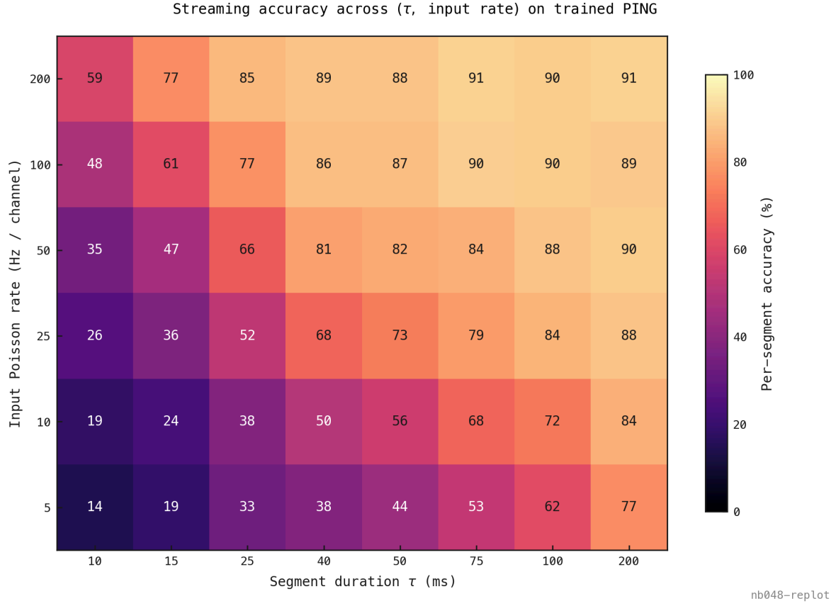
Figure 144: Per-segment accuracy over the full grid (3 seeds \times 1200 segments per cell). Three things stand out. (1) Sub-cycle failure below \tau \approx 15 ms: at \tau = 10 ms even 200 Hz input reaches only 59% — the network cannot classify within less than one cycle regardless of drive, the cleanest evidence that the gamma cycle is the temporal quantum of its classification ability. (2) Above one cycle, accuracy \approx f(\tau \cdot \text{rate}) : iso-accuracy contours run diagonal, so \tau and input rate substitute for each other — more drive compensates for shorter presentation and vice versa. (3) The trained operating point (200 ms, 25 Hz) sits at 88%, interior to the plateau — the corners gain only \approx 3 pp, so there is headroom in both directions.
