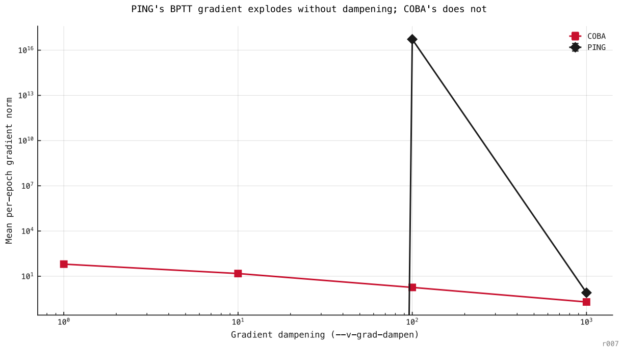
Figure 182: The mechanism: at low dampening PING's gradient norm blows up through the E \rightarrow I \rightarrow E loop, while COBA's stays bounded — which is why only PING's accuracy collapses.
