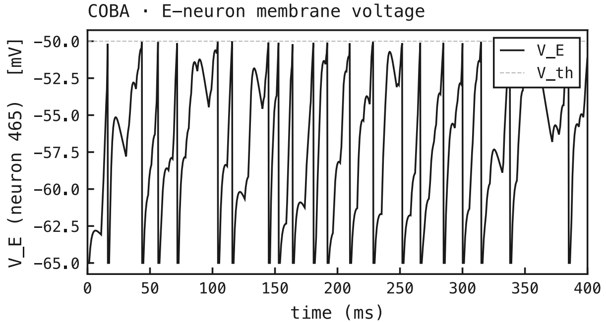
Figure 24: Membrane voltage V_E (black) of the most active E cell, recurrent loop off (COBA, ei-strength 0). Driven only by feedforward input, the cell charges toward threshold ( V_{th} = -50 mV, faint dashed) and hard-resets to V_{reset} = -65 mV each time it fires — irregular, input-paced spiking with no rhythmic structure. The rhythm-free control for Figure 3a.
